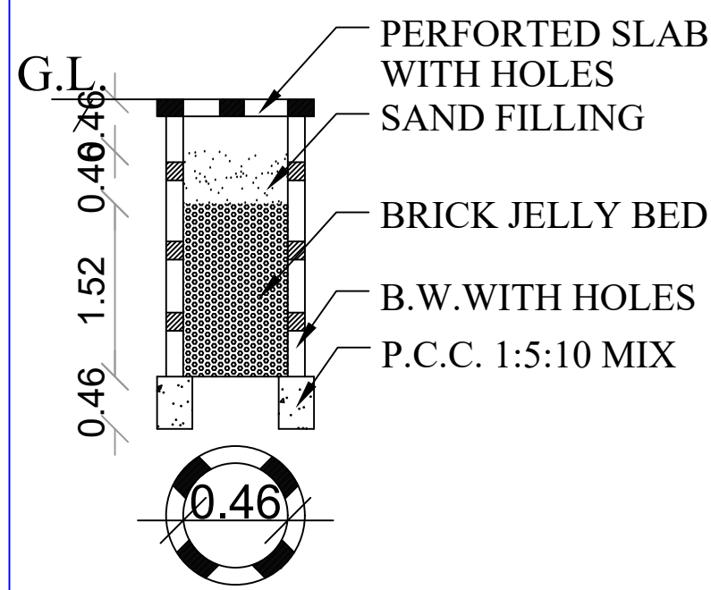
PERCOLATION PIT
