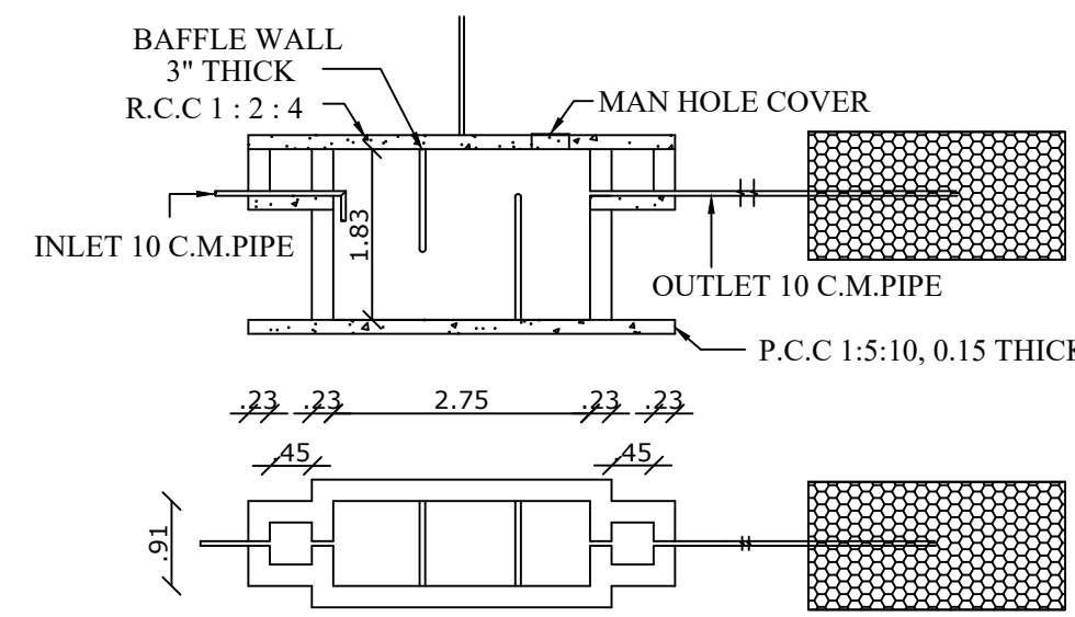
SEPTIC TANK & TRENCH
