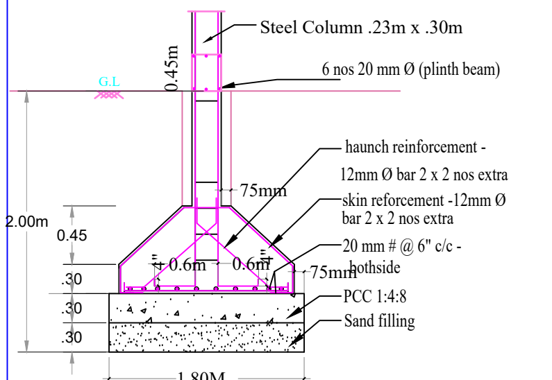
FOUNDATION - PROVIDED WITH EARTHQUAKE RESISTANT DESIGN OF STRUCTURES AS PER IS AND N B C NORMS.
