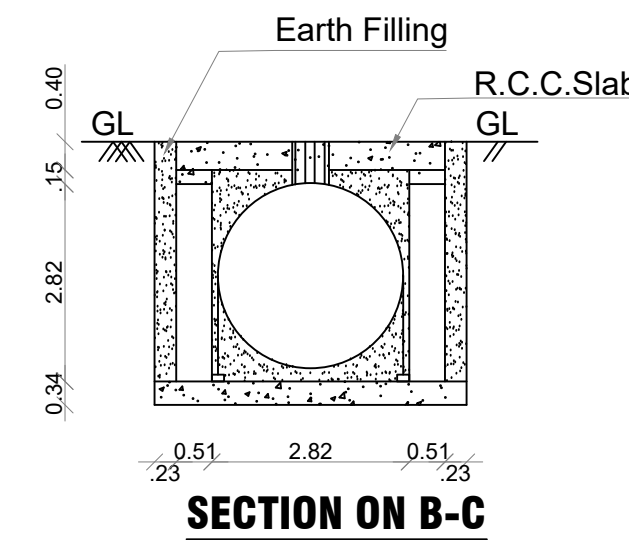
SECTION ON B-C
