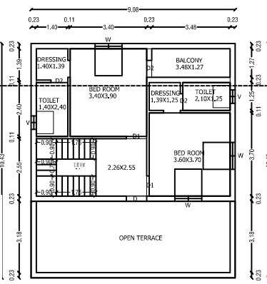
FIRST FLOOR PLAN (PROPOSED)
