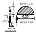
PARAPET WALL
