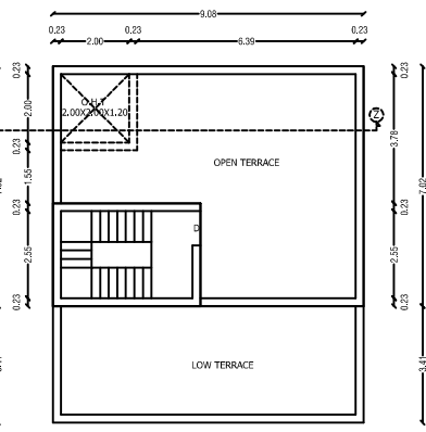
TERRACE FLOOR PLAN (PROPOSED)
