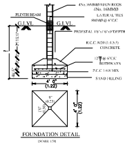
FOUNDATION DETAIL (SCALE: 1/8)
