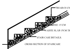
CROSS SECTION OF STAIRCASE
