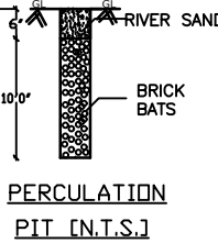
FOUNDATION DETAILS
