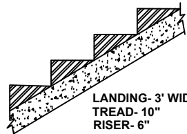
STAIR DETAIL
