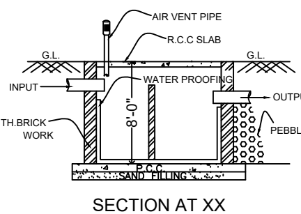
SECTION AT XX
