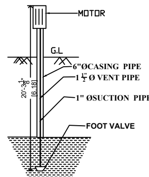
SEC. OF BOREWELL
