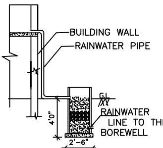
SEC. OF RAIN WATER HARVEST
