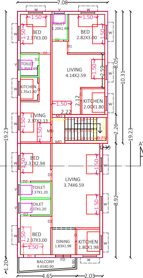
SECOND FLOOR SCALE 1:100
