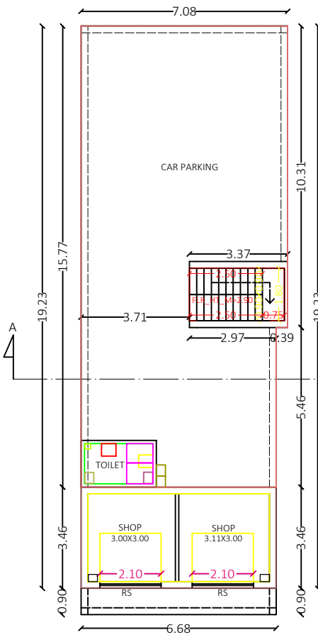
GROUND FLOOR SCALE 1:100
