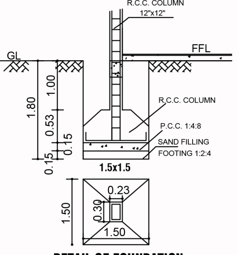
DETAIL OF FOUNDATION Not to Scale
