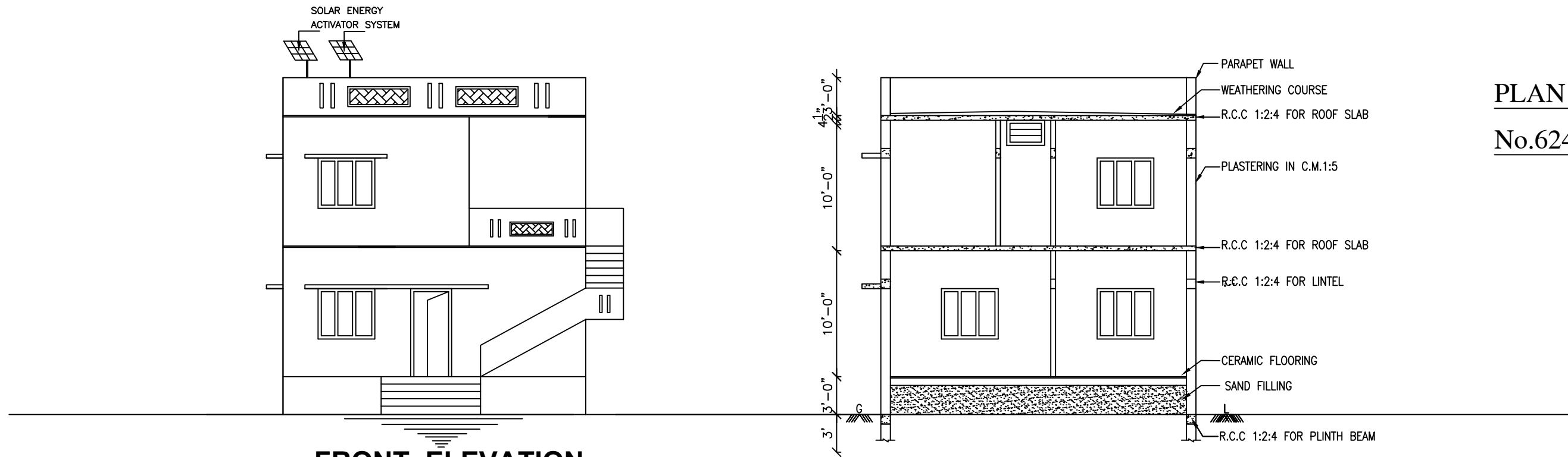
FRONT ELEVATION
