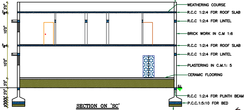
SECTION ON 'SC'
