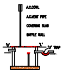
SEPTIC TANK DETAILS
