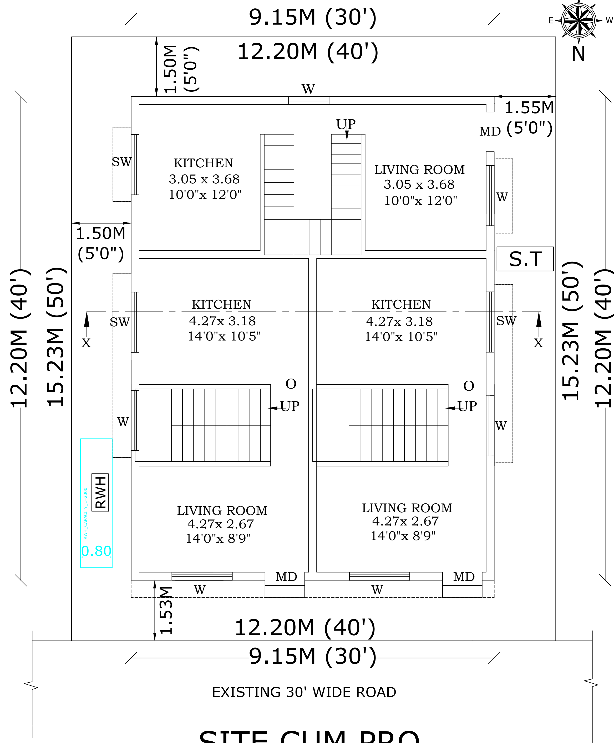
SITE CUM PRO. GROUND FLOOR PLAN
