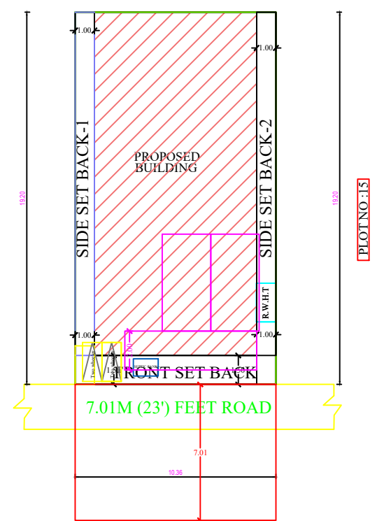
SITE PLAN
