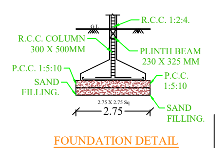
FOUNDATION DETAIL
