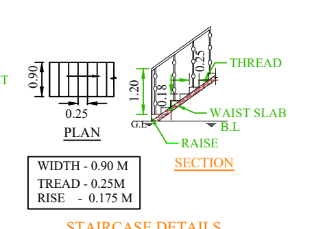
STAIRCASE DETAILS
