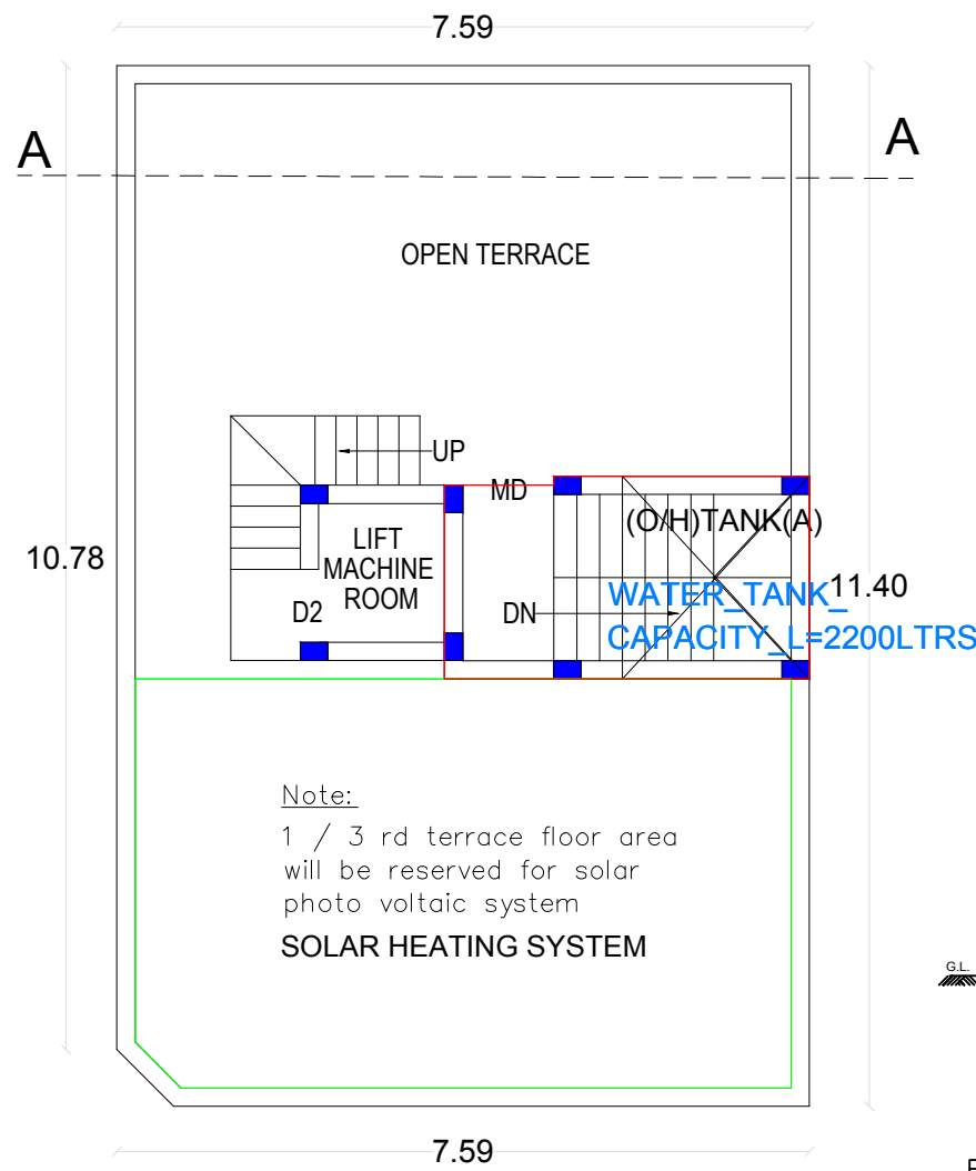
PRO. TERRACE FLOOR PLAN
