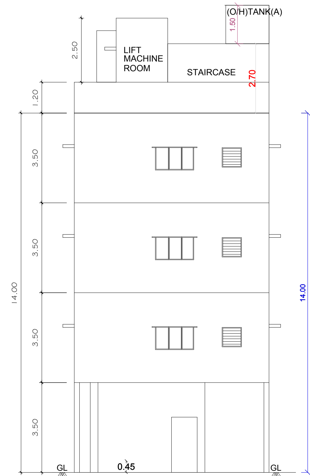
FRONT ELEVATION
