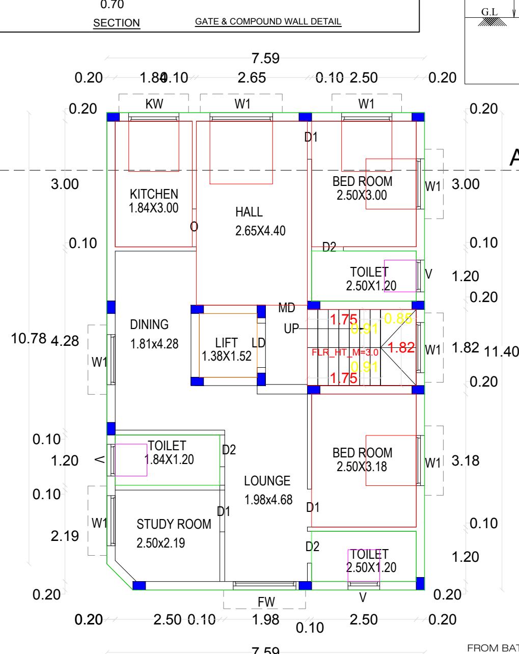
PRO. THIRD FLOOR PLAN
