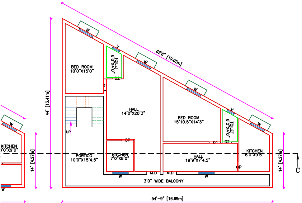
PRO.FIRST FLOOR PLAN
