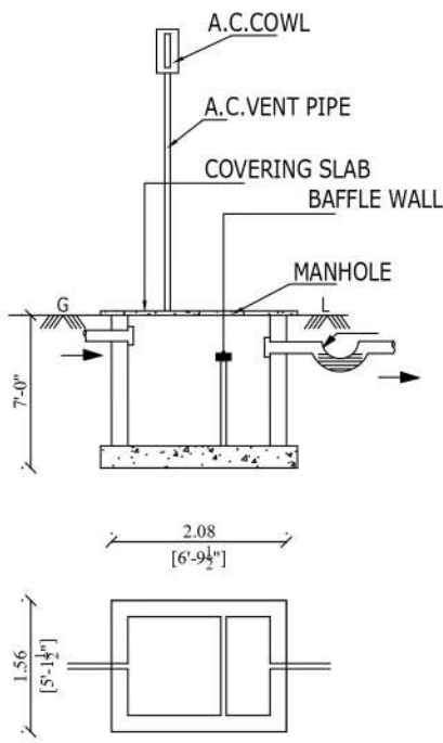
SEPTIC TANK
