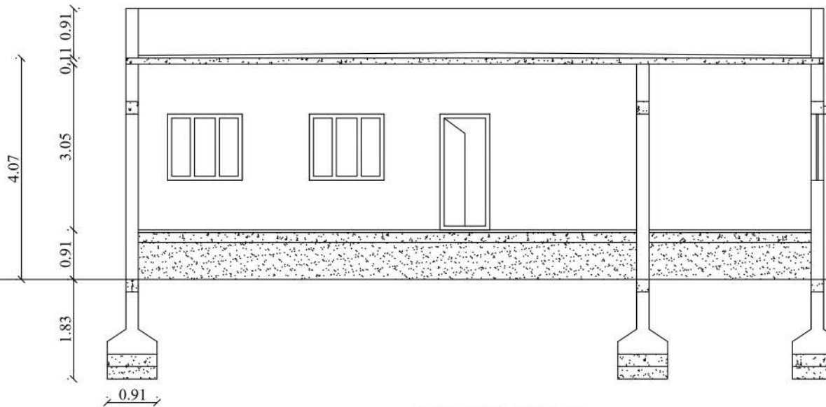
SECTION ON 'LS'
