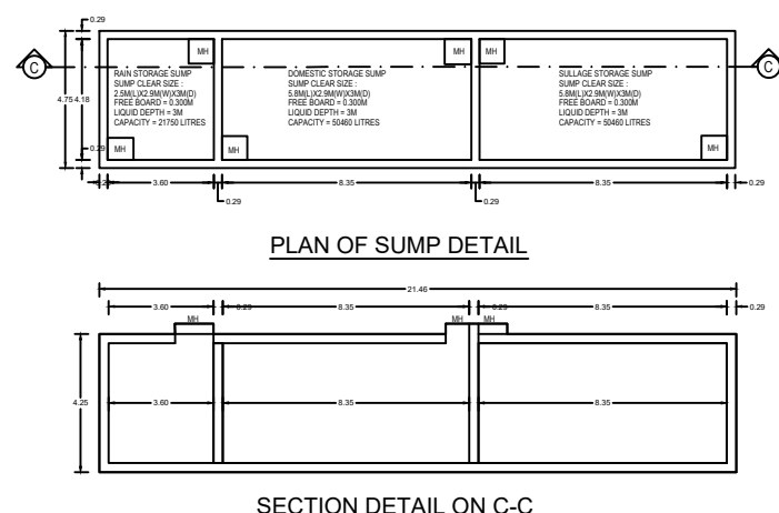
SECTION DETAIL ON C-C
