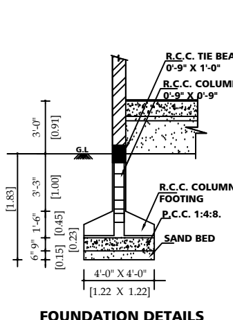
FOUNDATION DETAILS
