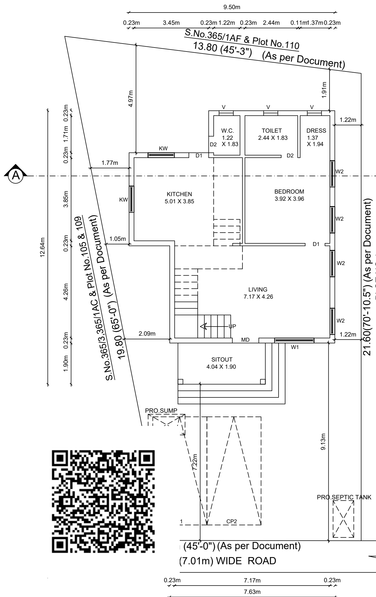
SITE CUM PRO. GROUND FLOOR PLAN
