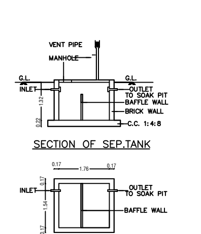
PLAN SEPTIC. TANK
