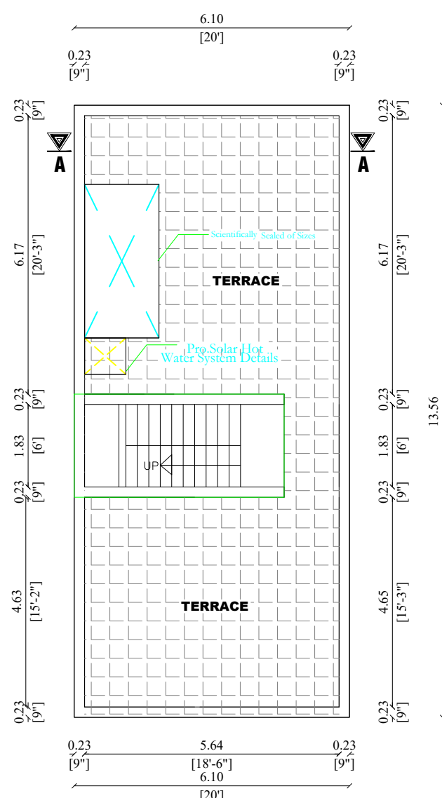
PRO.TERRACE FLOOR PLAN
