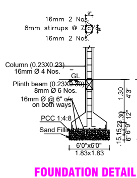
FOUNDATION DETAIL
