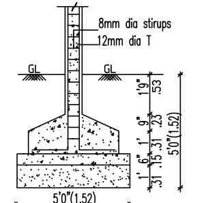
COLUMN FOUNDATION DETAIL SCALE 1"=4'0" (1:50)
