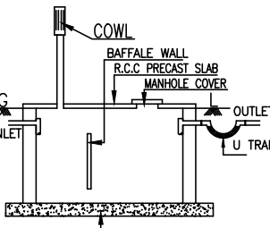
SECTION 1:5:10 DETAILS OF SEPTIC TANK
