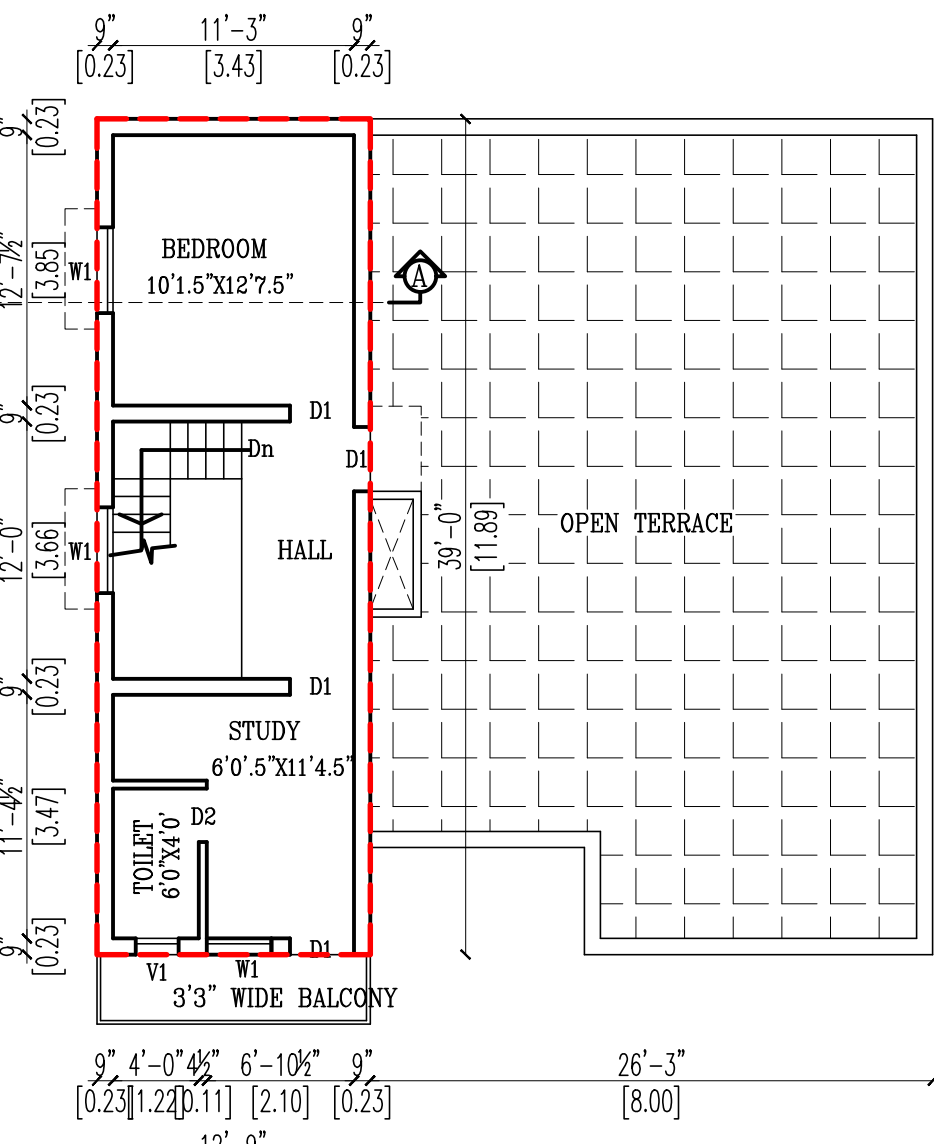
PRO. SECOND FLOOR PLAN
