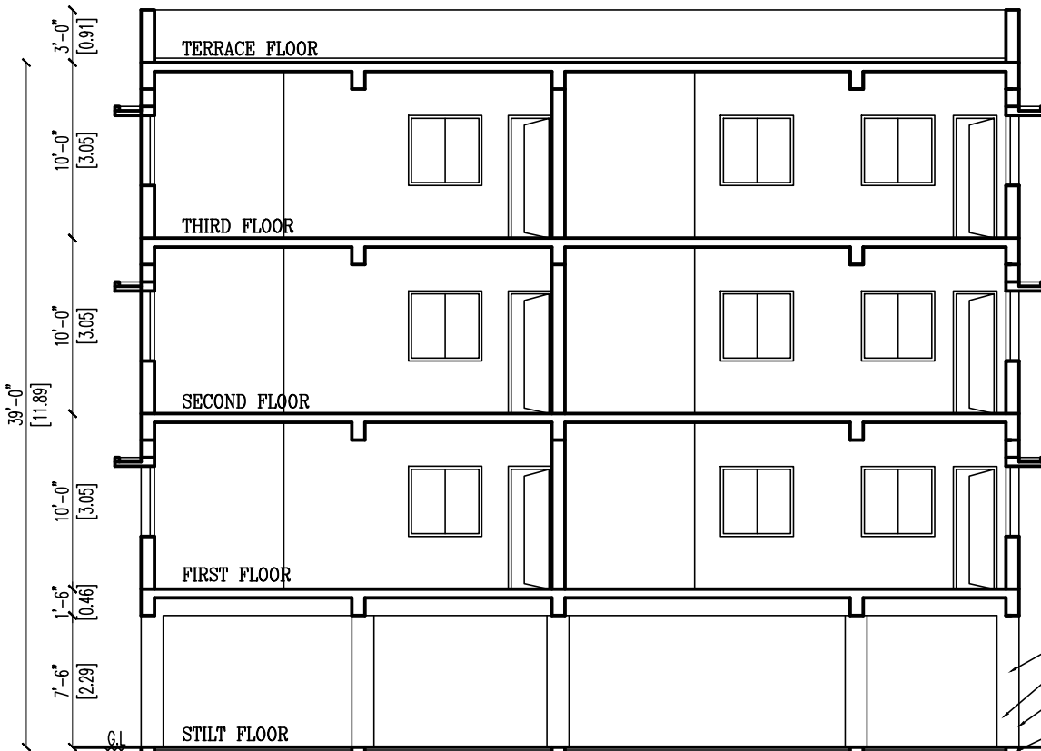
SECTION - AA
