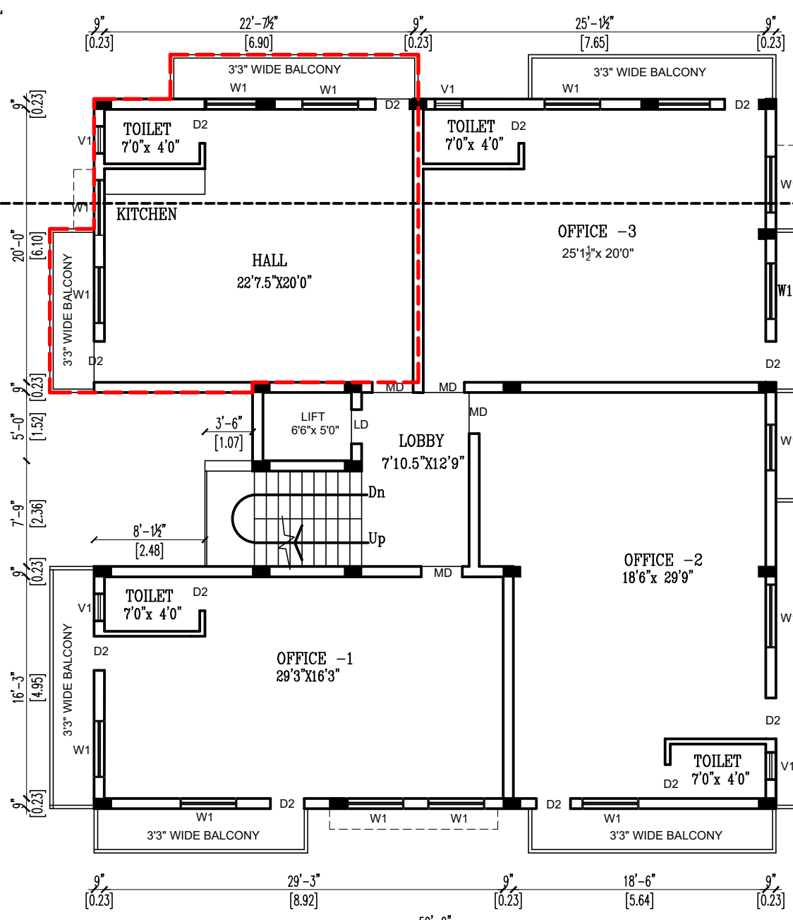
EXTG. FIRST FLOOR (COMMERCIAL)/ PRO. ADDITIONAL FIRST FLOOR PLAN (RESIDENTIAL)
