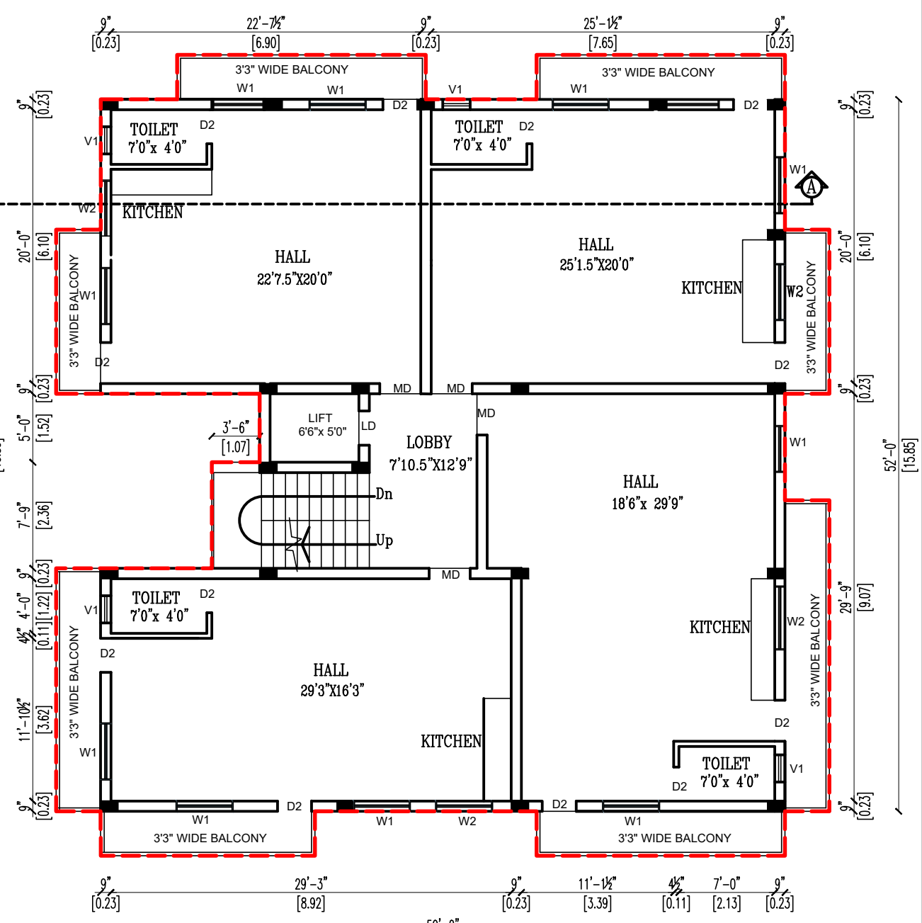
PRO. SECOND / THIRD FLOOR PLAN (RESIDENTIAL)
