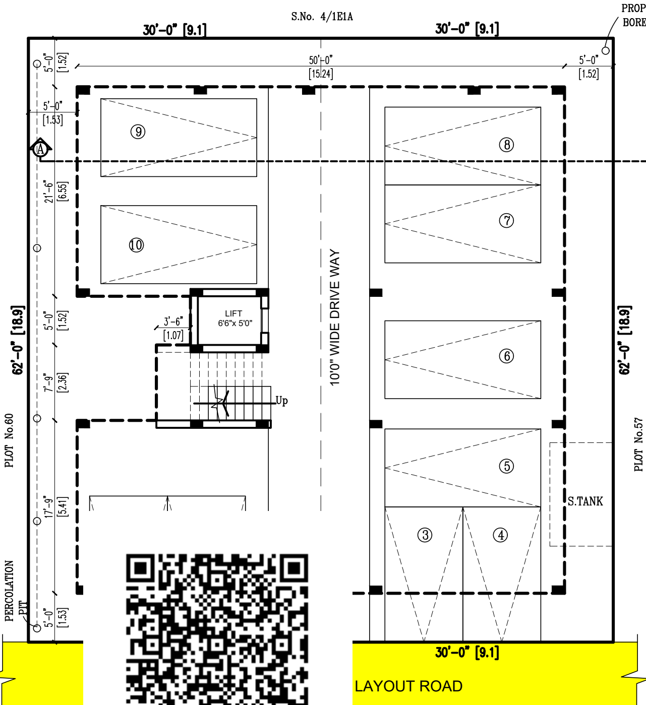
FLOOR PLAN
