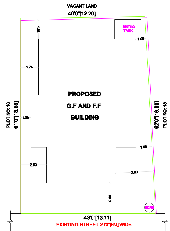
SITE & PROPOSED PLAN
