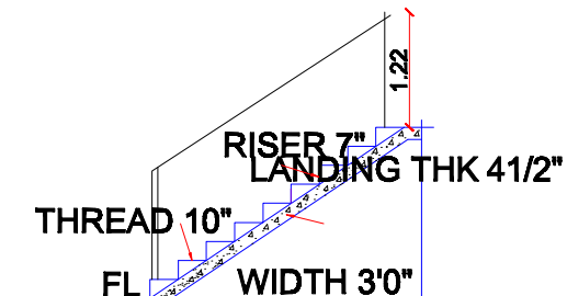
SEC. OF STAIR CASE DETAILS
