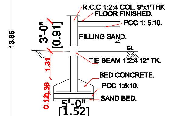
COLUMN FOUNDATION
