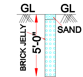
PERCOLATION PIT
