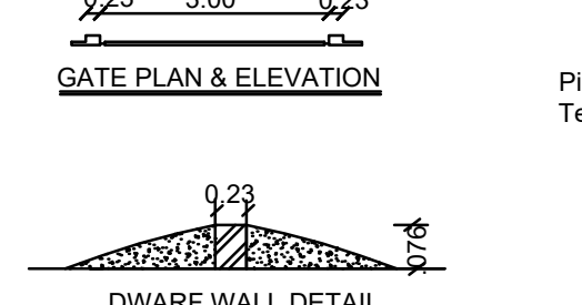
DWARF WALL DETAIL
