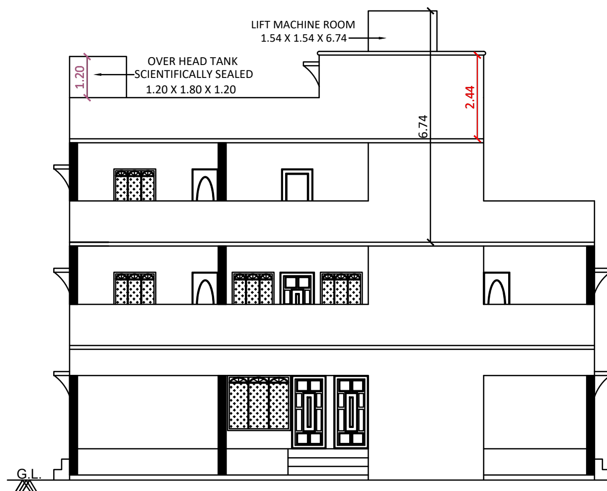
FRONT ELEVATION
