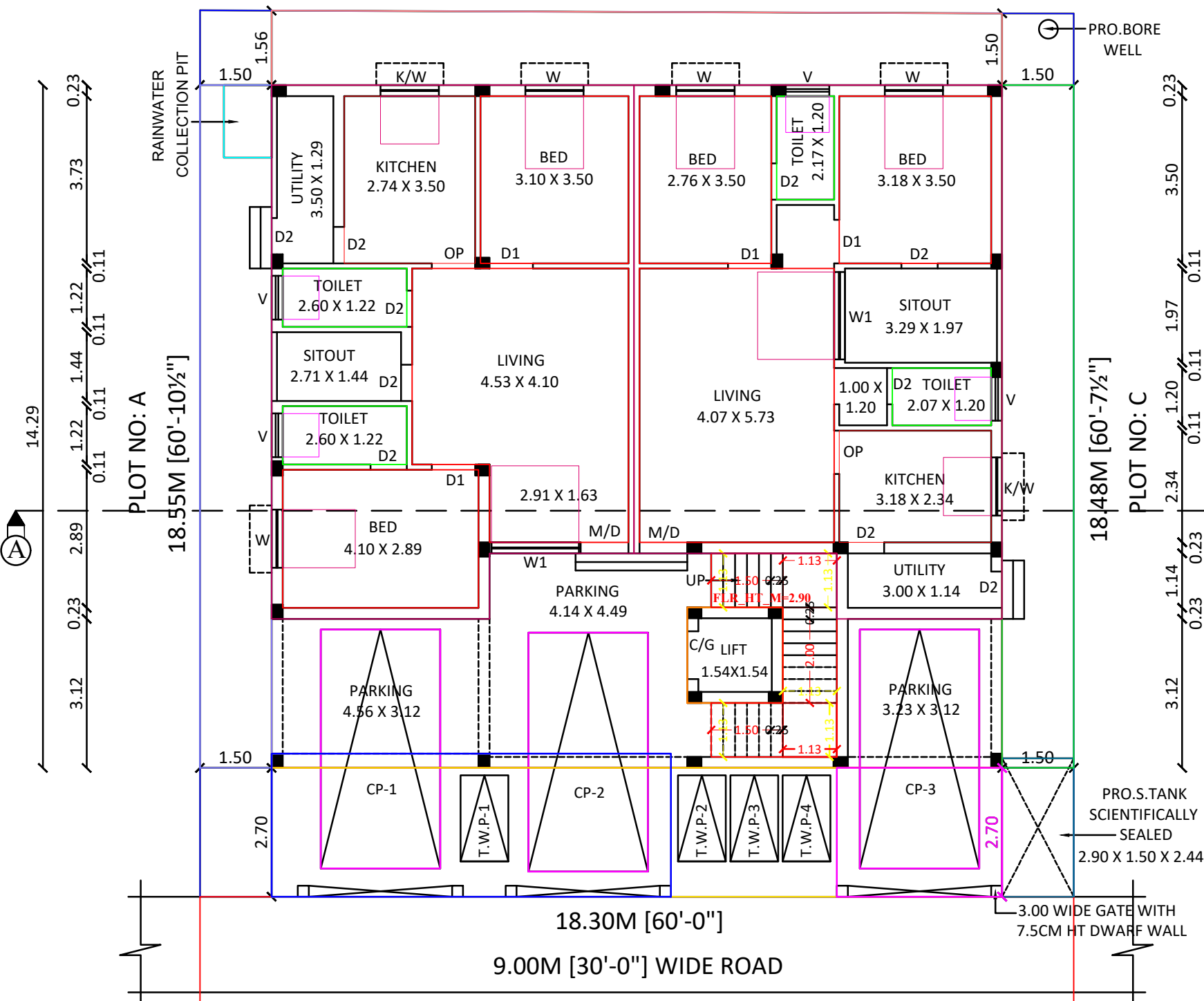
SITE CUM PRO.GROUND FLOOR PLAN
