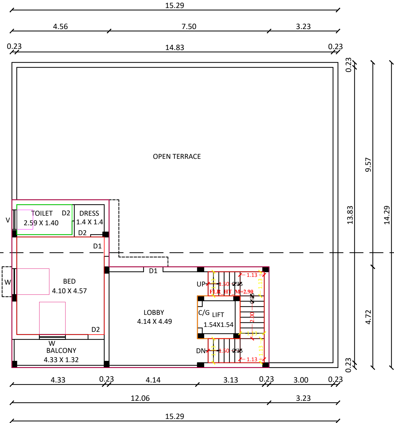
PRO.SECOND FLOOR(PT) PLAN
