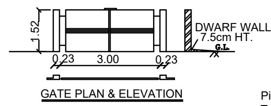
GATE PLAN & ELEVATION
