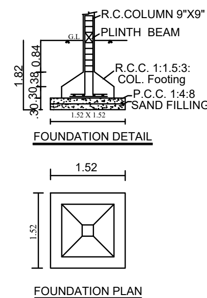
FOUNDATION PLAN
