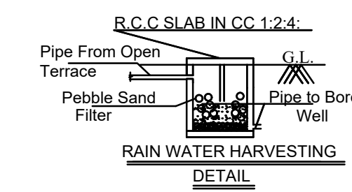
RAIN WATER HARVESTING DETAIL
