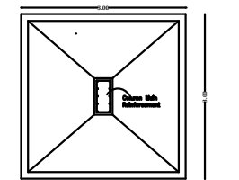
COLUMN FOUNDATION DETAIL PLAN OF FOOTING
