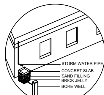
DETAIL RAINWATER HARVESTING
