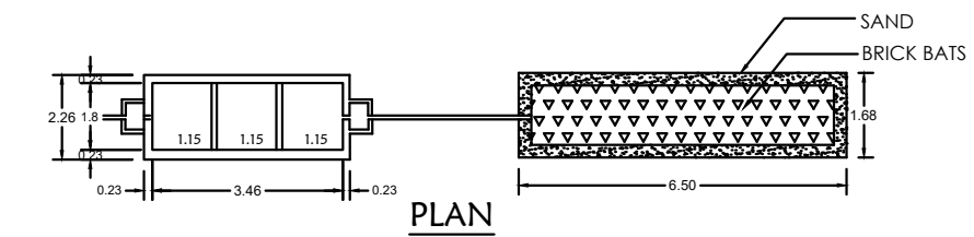
PLAN SEPTIC TANK AND TRENCH
