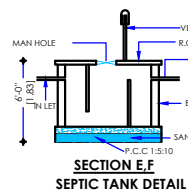
SECTION E-F SEPTIC TANK DETAIL
