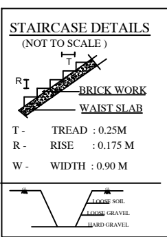
STAIRCASE DETAILS (NOT TO SCALE)
