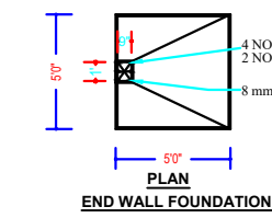
END WALL FOUNDATION
