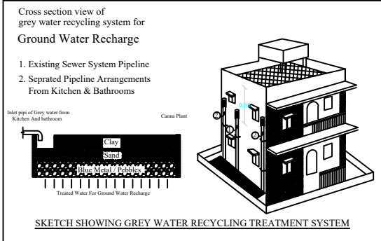
SKETCH SHOWING GREY WATER RECYCLING TREATMENT SYSTEM
