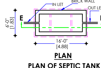
PLAN PLAN OF SEPTIC TANK
