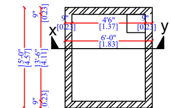
U.G.SUMP-PLAN HERMITICALLY SEALED
