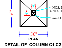
DETAIL OF COLUMN C1,C2
