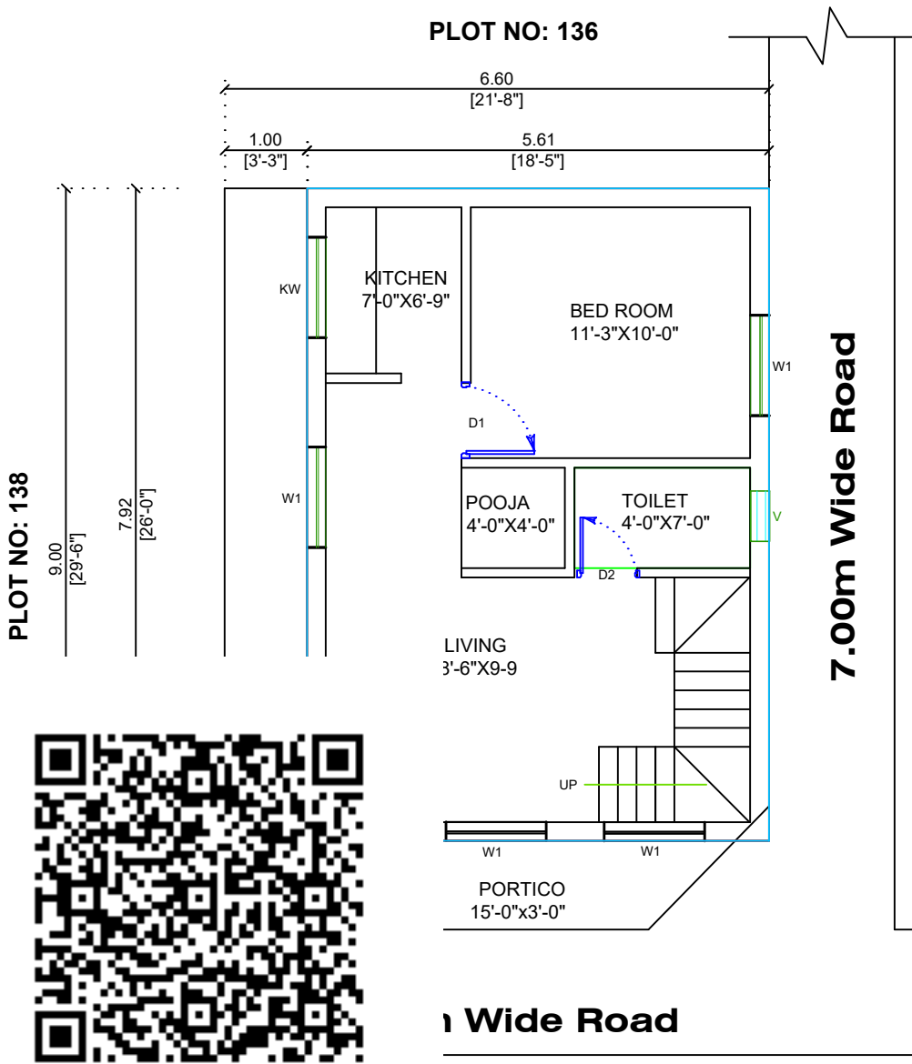
SITE CUM GROUND FLOOR PLAN
