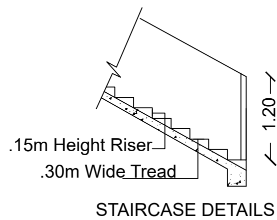
STAIRCASE DETAILS
