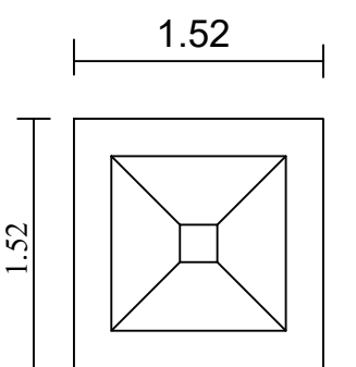
FOUNDATION PLAN
