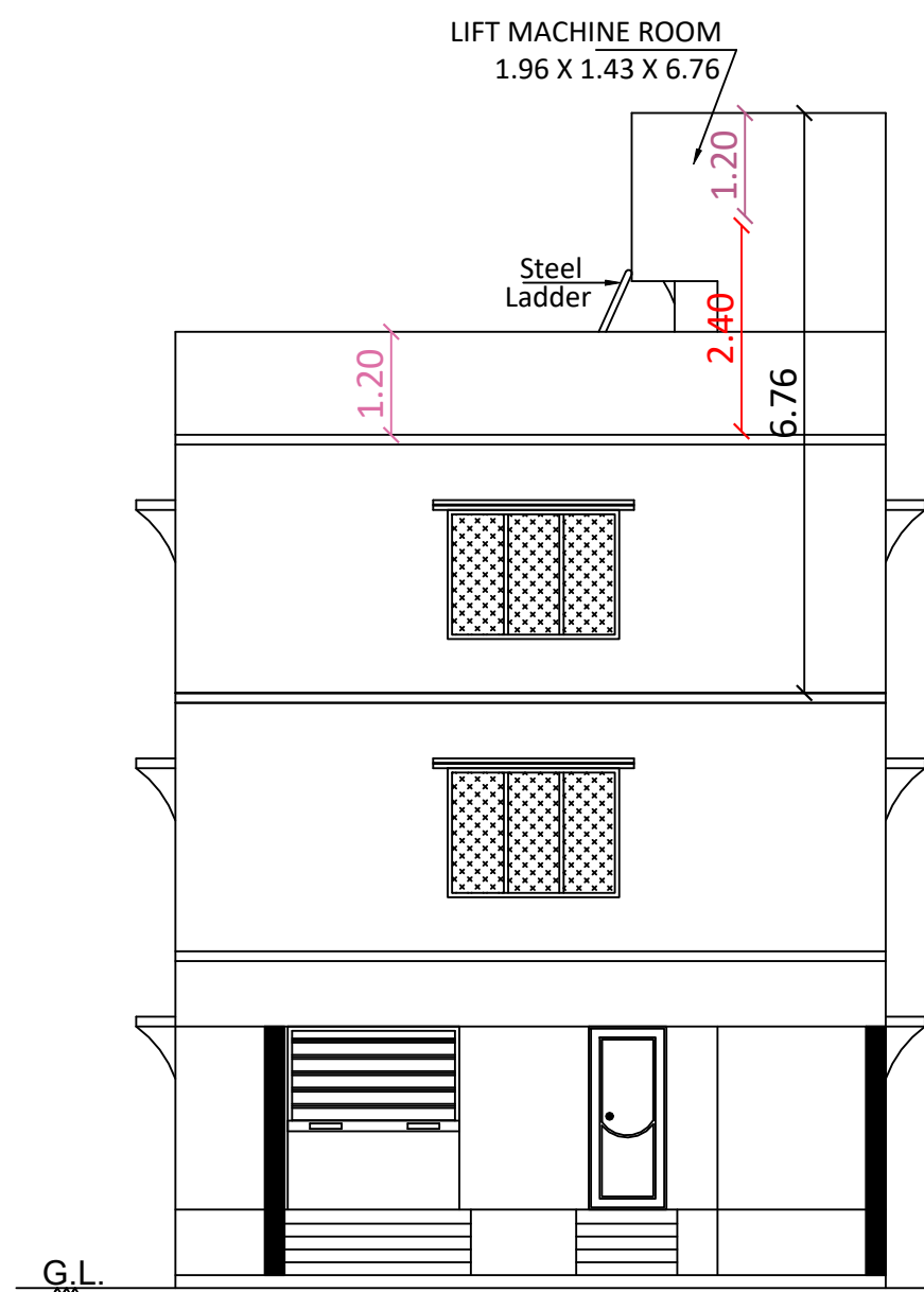
FRONT ELEVATION
