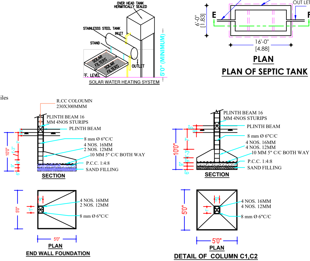
DETAIL OF COLUMN C1,C2
