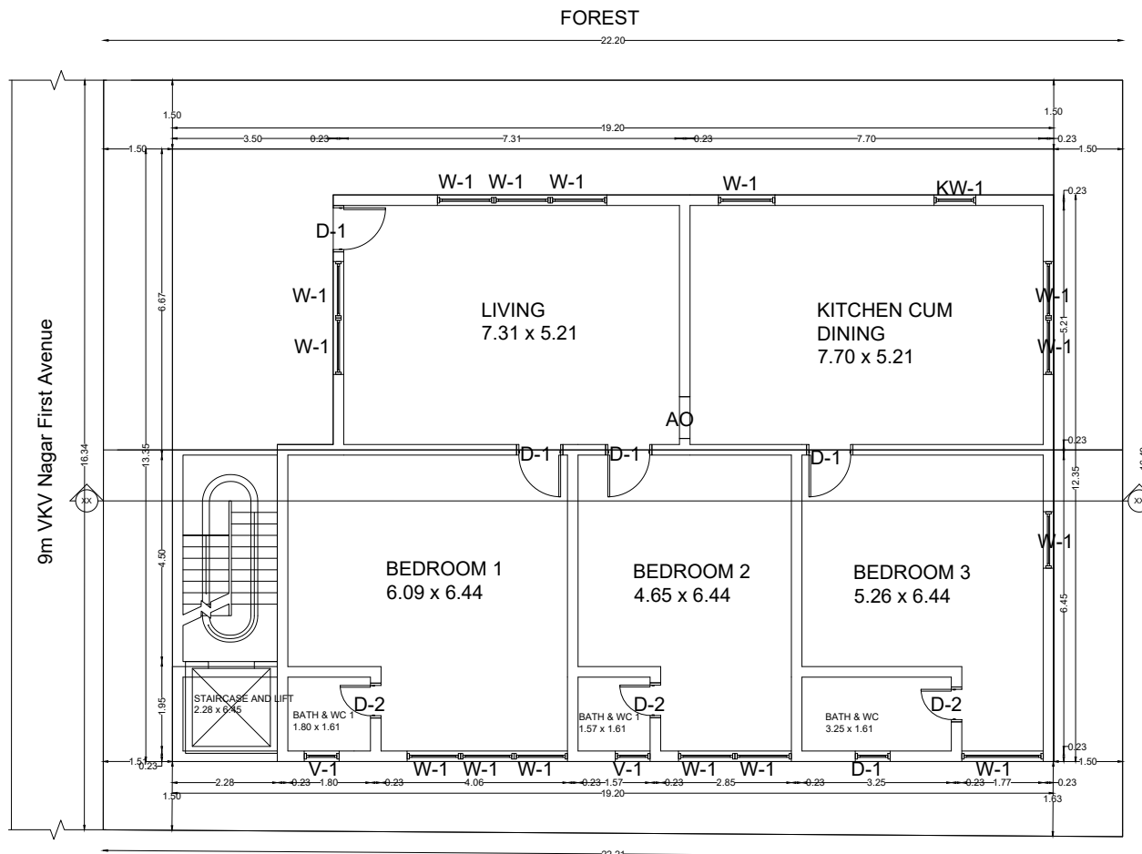
SITE CUM GROUND FLOOR PLAN MIDHUN PRABHU PLOT
