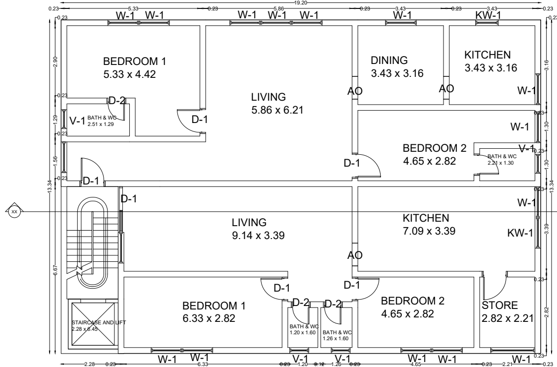
TYPICAL FIRST FLOOR AND SECOND FLOOR PLAN
