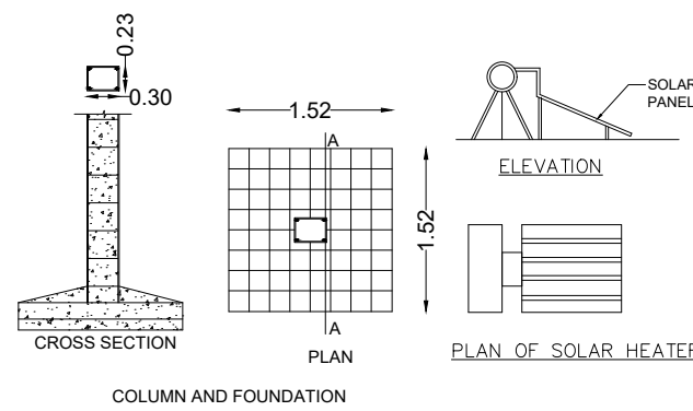
COLUMN AND FOUNDATION
