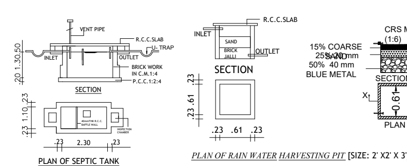
PLAN OF RAIN WATER HARVESTING PIT (SIZE: 2' X 2' X 3')
