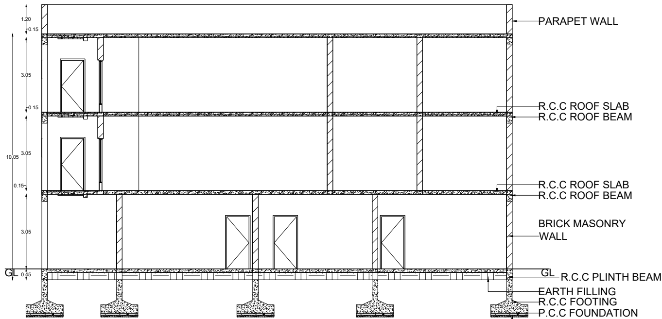
SECTION XX - XX
