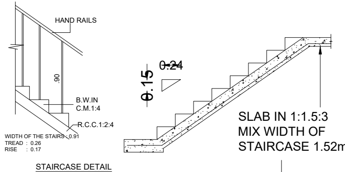
STAIRCASE DETAIL
