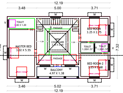
PROPOSED FIRST FLOOR
