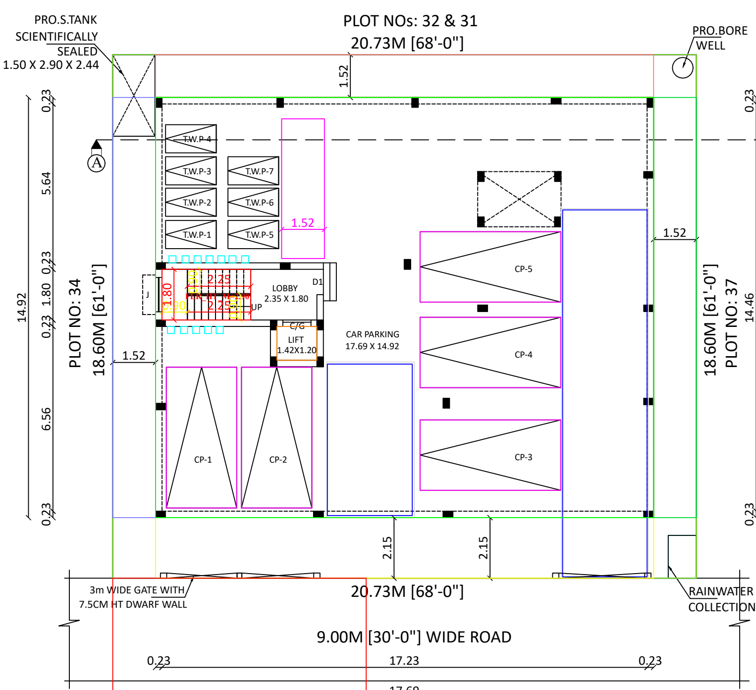
SITE CUM PRO.STILT FLOOR PLAN
