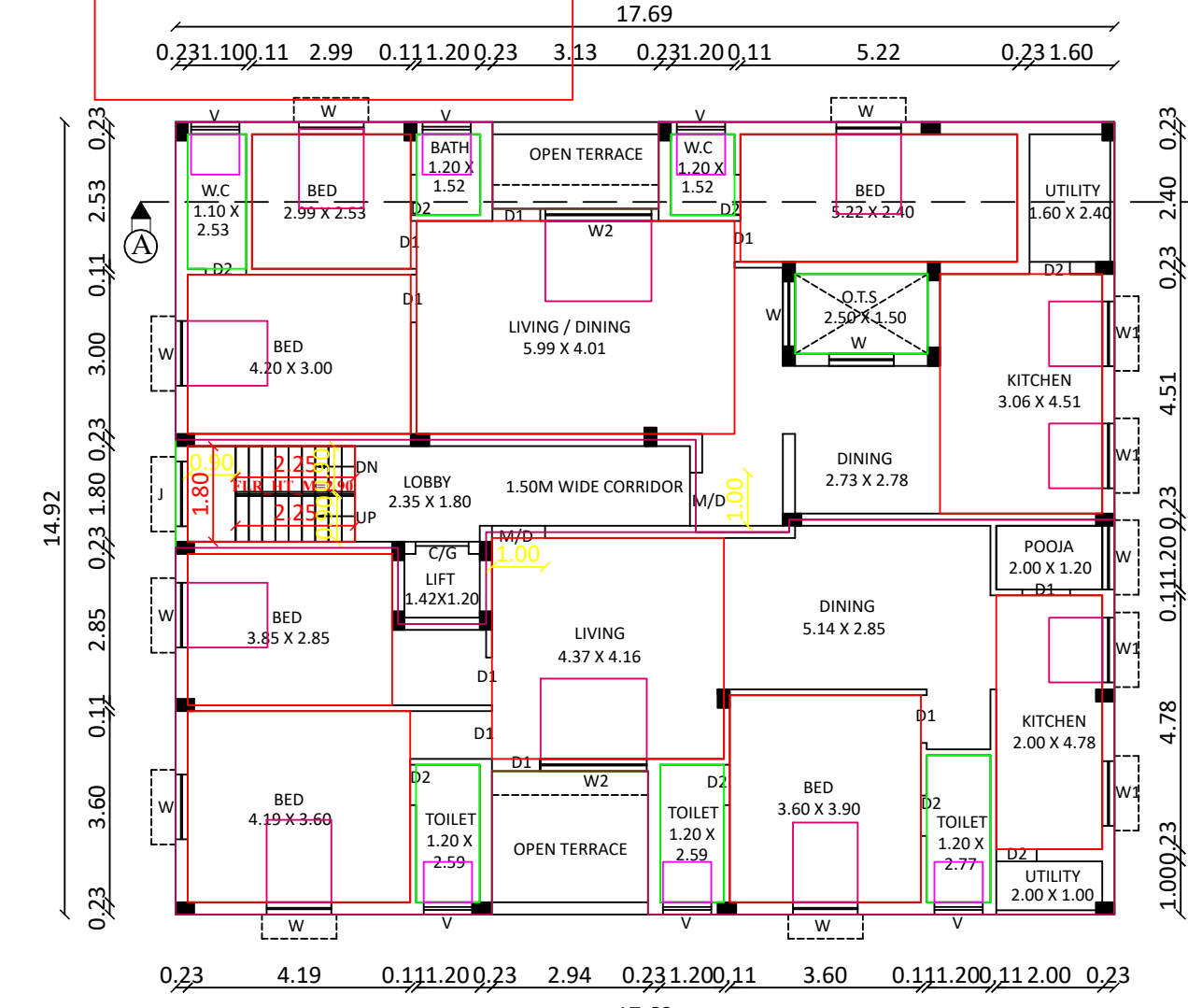
PRO.THIRD FLOOR(PT) PLAN
