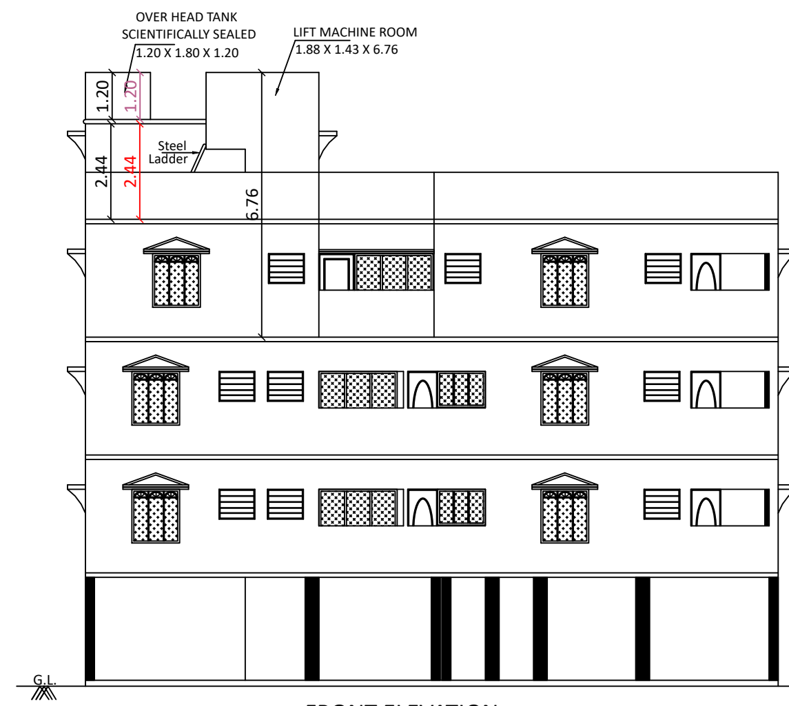
FRONT ELEVATION
