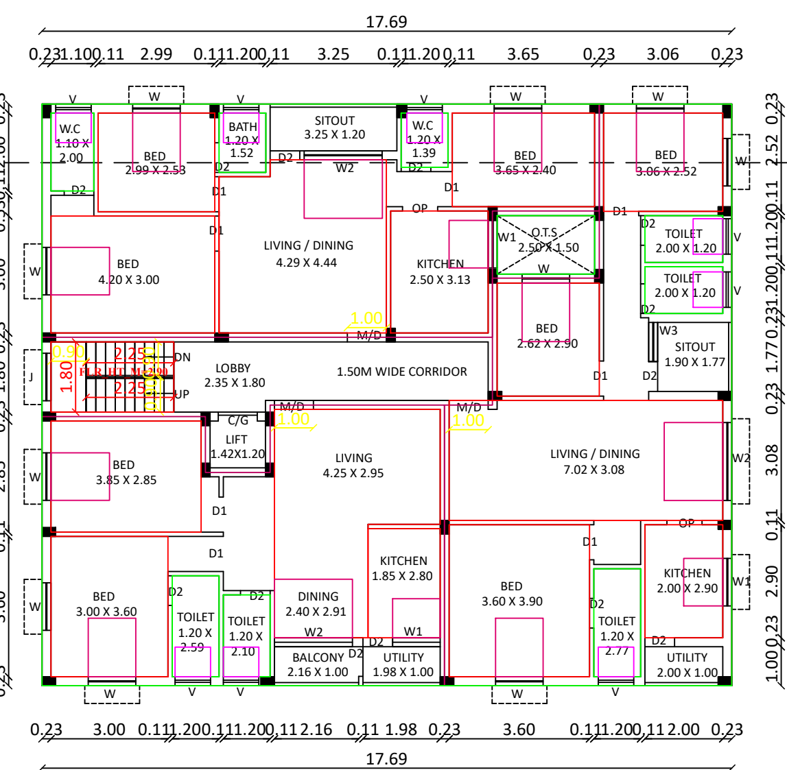
PRO.SECOND FLOOR PLAN
