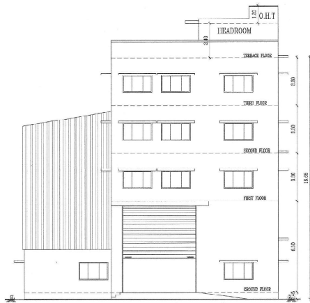
FRONT ELEVATION (WEST SIDE)
