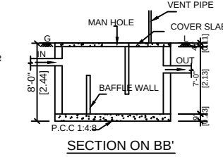
SECTION ON BB'
