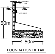
FOUNDATION DETAIL
