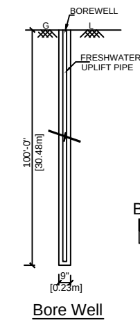
Bore Well
