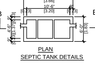
PLAN OF SEPTIC TANK DETAILS
