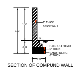
SECTION OF COMPOUND WALL
