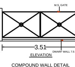
COMPOUND WALL DETAIL SCALE = 1: 50
