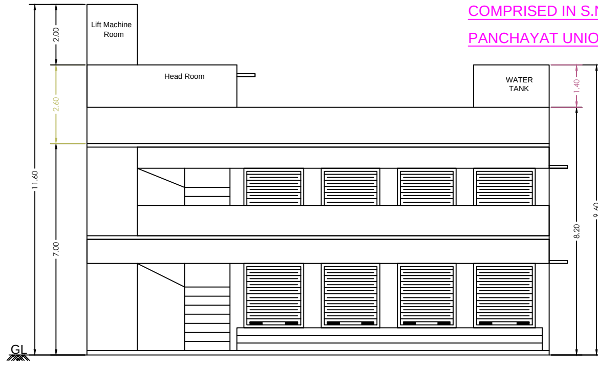
FRONT ELEVATION.
