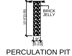
PERCOLATION PIT
