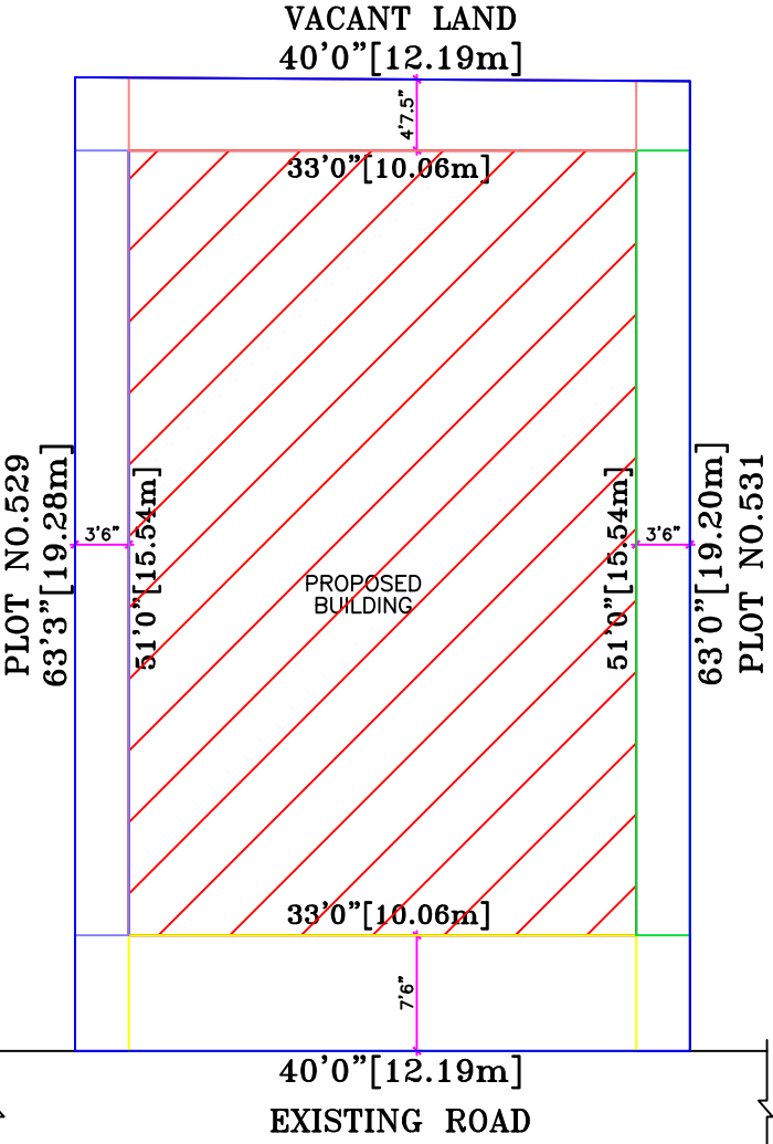
SITE PLAN SCALE 1"=8'0"
