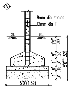
COLUMN FOUNDATION DETAIL
