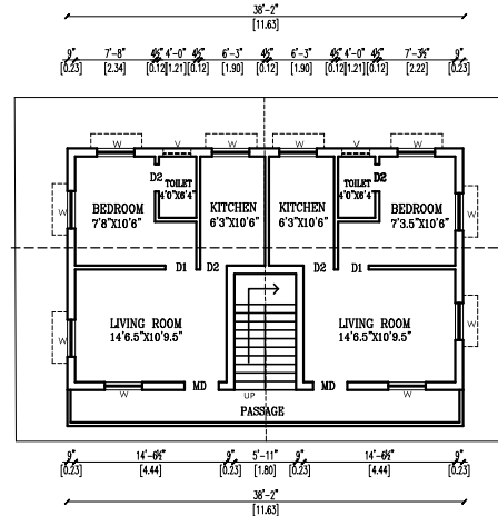
TYPICAL 1st, 2nd & 3rd FLOOR
