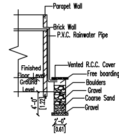
SECTION OF RAINWATER HARVESTING SYSTEM
