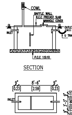
DETAILS OF SEPTIC TANK
