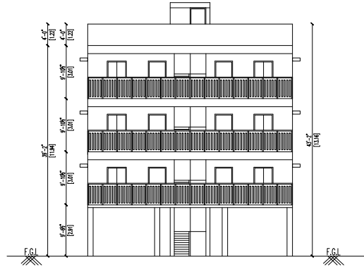
FRONT ELEVATION
