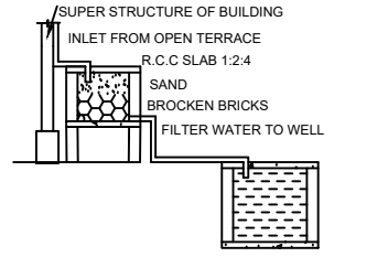
RAINWATER HARVESTING
