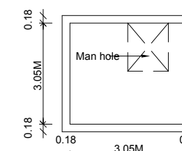
SUMP DETAILS
