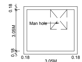
DRINKING WATER SUMP DETAILS
