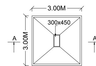
PLAN OF FOOTING Footling Detail
