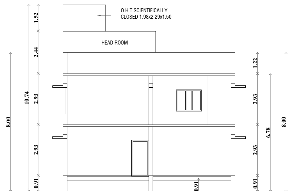
SECTION ON A-A PROPOSED
