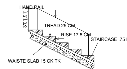
STAIRCASE DETAILS
