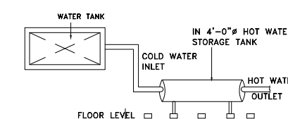
SOLAR HOT WATER SYSTEM DETAIL Solar Waterheater Detail
