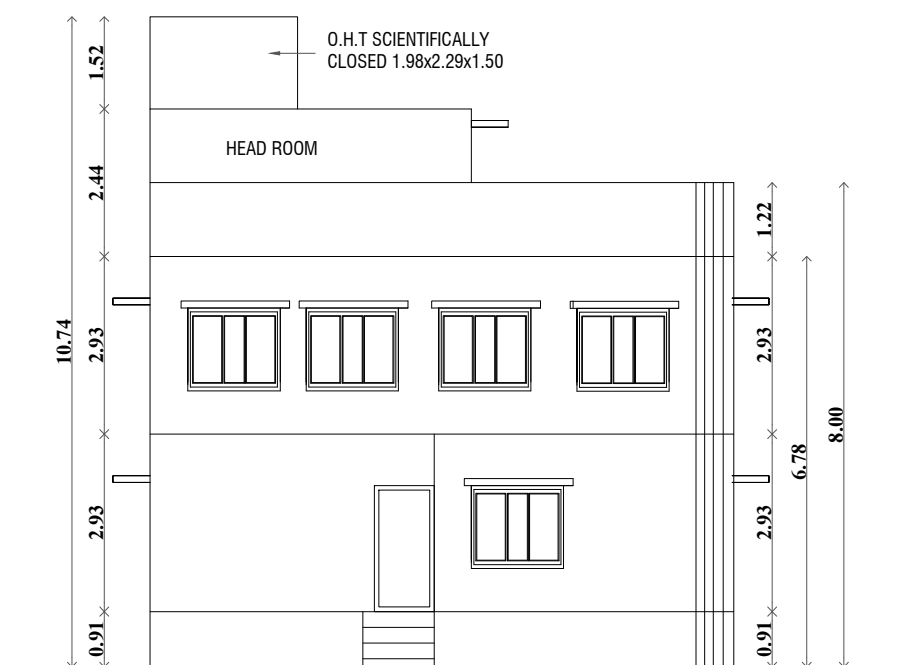
ELEVATION PROPOSED
