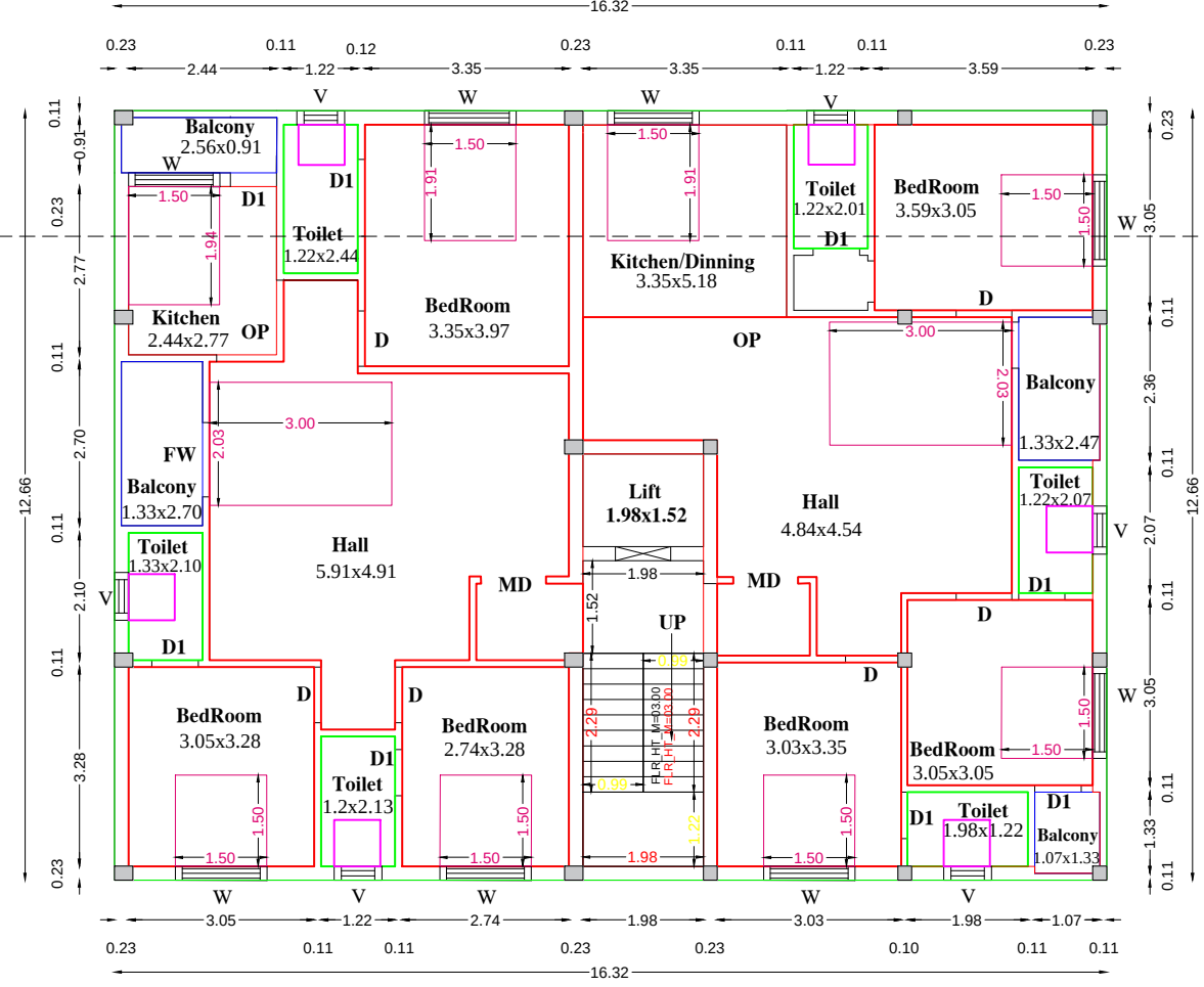
FLOOR01
