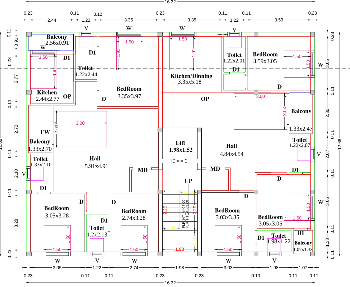
FLOOR03
