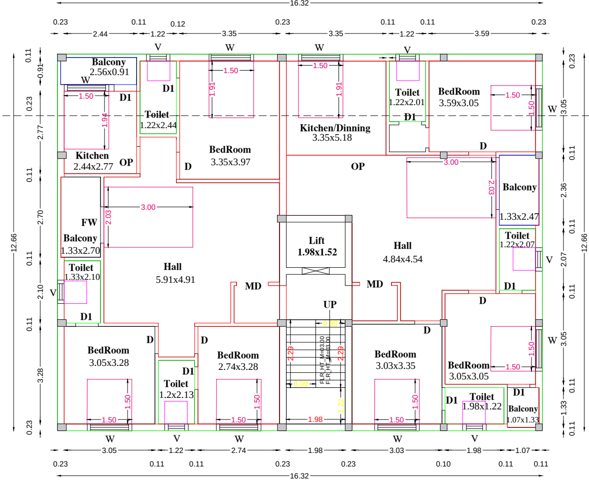
FLOOR02
