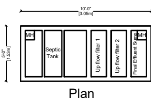
Septic tank with upflow filter system
