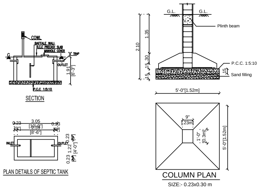
TYPICAL FOUNDATION DETAIL Footing Detail
