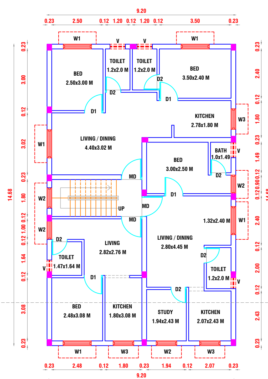
TYPICAL FIRST & SECOND FLOOR PLAN
