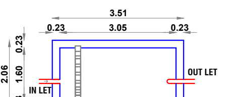
PLAN OF SEPTIC TANK CAPACITY - 8000 LITRES
