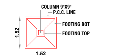
PLAN OF FOOTING
