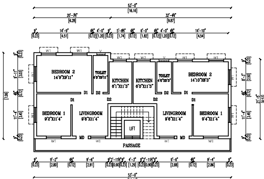
TYPICAL 1st, 2nd & 3rd FLOOR
