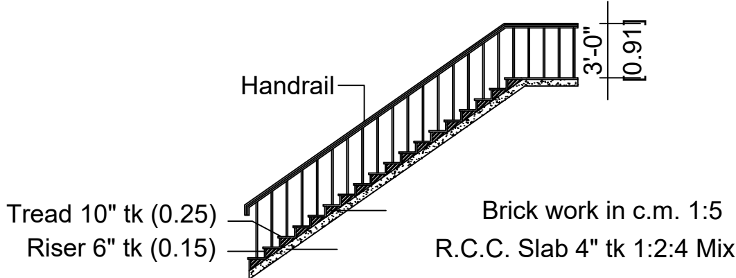
Staircase Details
