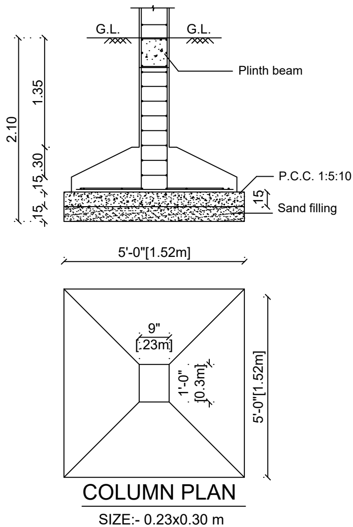
TYPICAL FOUNDATION DETAIL Footing Detail
