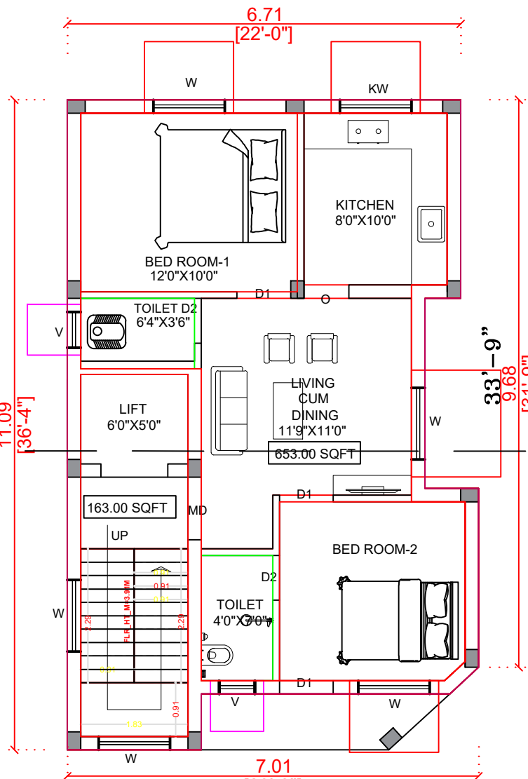
TYPICAL I, II & III-rd FLOOR PLAN
