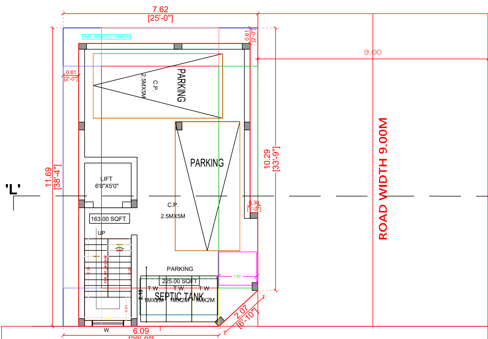
SITE CUM STILT FLOOR PLAN
