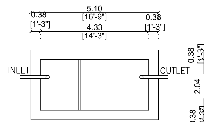
PLAN DETAILS OF SEPTIC TANK
