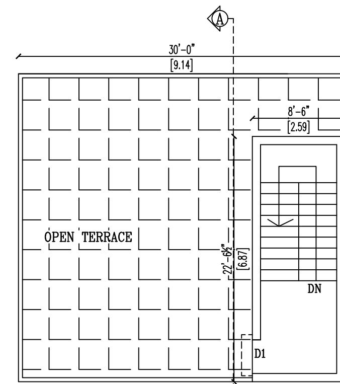
PRO. TERRACE FLOOR PLAN
