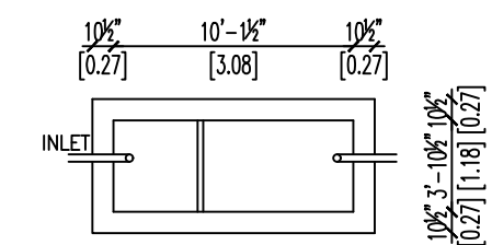
DETAILS OF SEPTIC TANK
