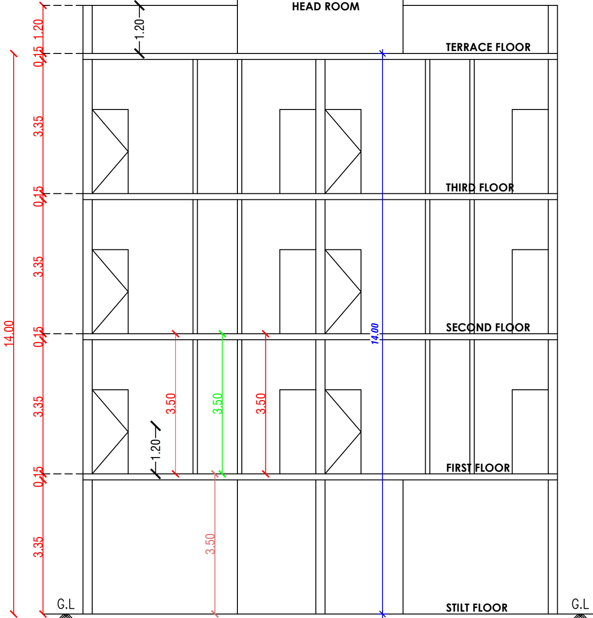
SECTION 'X-X' (PROPOSED)
