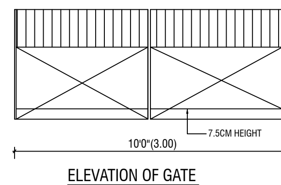
ELEVATION OF GATE
