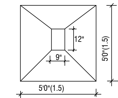
PLAN FOUNDATION DETAIL
