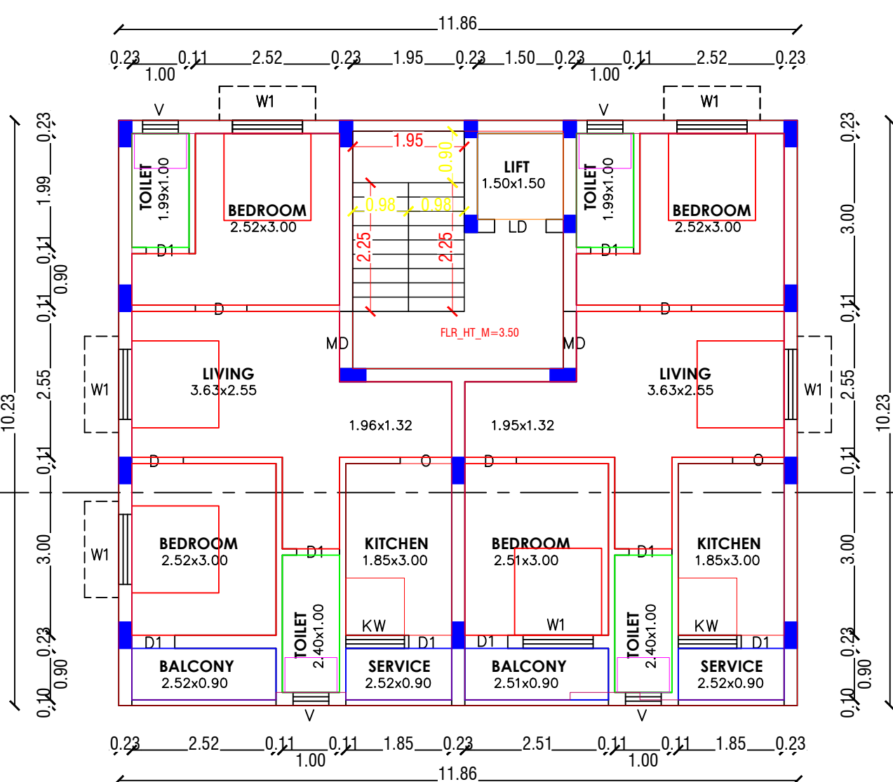
FIRST, SECOND & THIRD FLOOR PLAN (PROPOSED)
