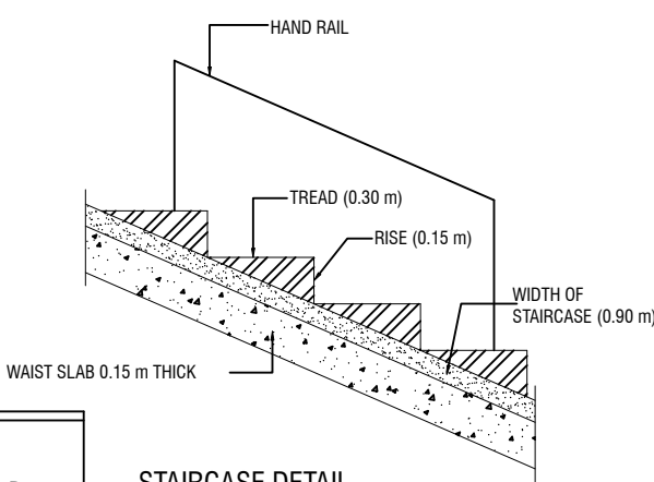
STAIRCASE DETAIL
