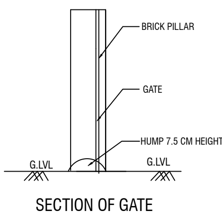
SECTION OF GATE
