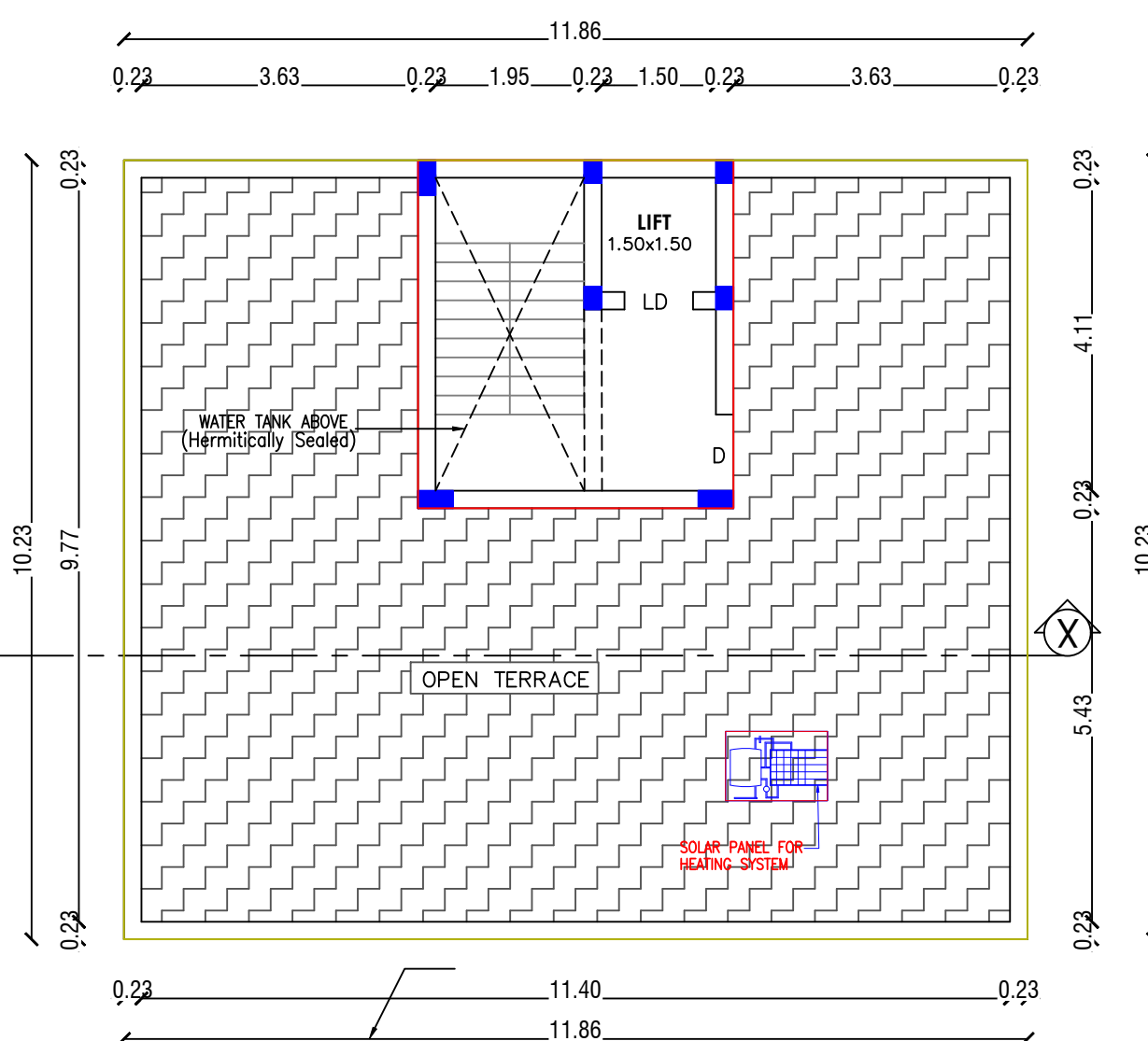
TERRACE FLOOR PLAN (PROPOSED)
