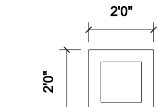
PERCOLATION PIT
