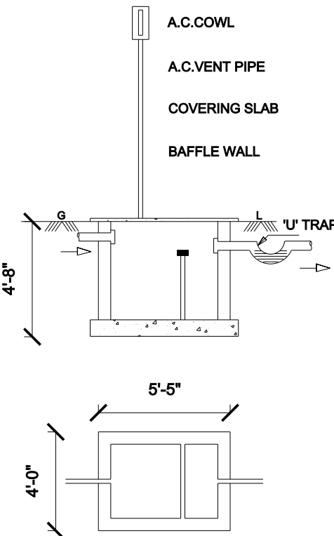
SEPTIC TANK
