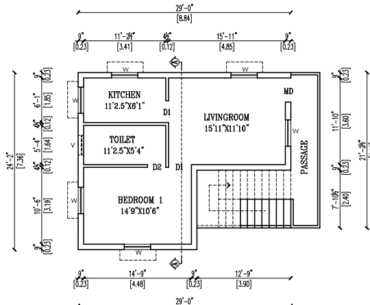
TYPICAL SECOND AND THIRD FLOOR PLAN
