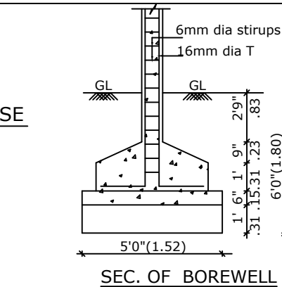
SEC. OF BOREWELL
