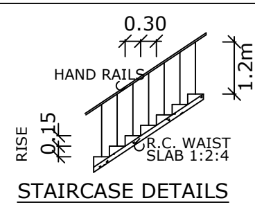
STAIRCASE DETAILS
