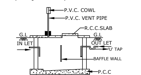
SEC. OF SEPTIC TANK
