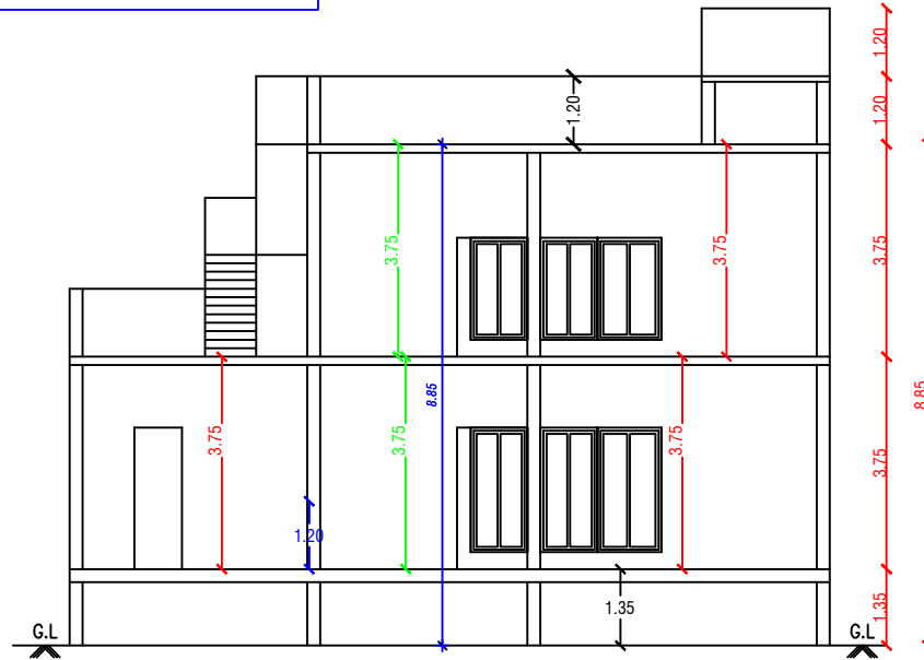
SECTION 'X-X' (PROPOSED)
