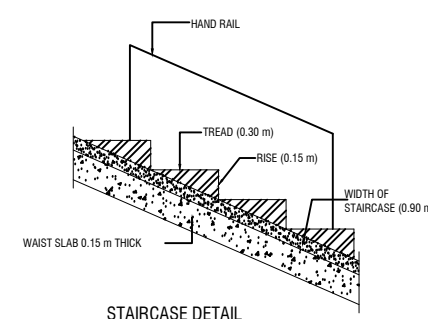
STAIRCASE DETAIL
