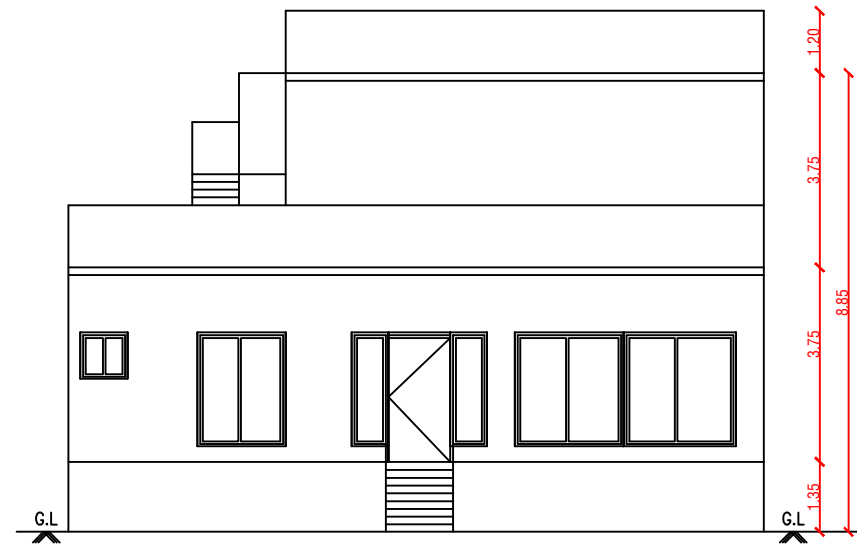
FRONT ELEVATION (PROPOSED)
