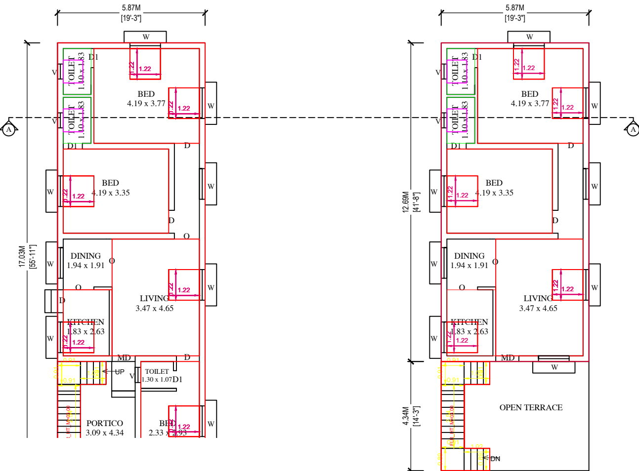
PLAN
