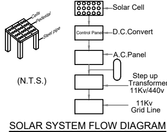
SOLAR SYSTEM FLOW DIAGRAM
