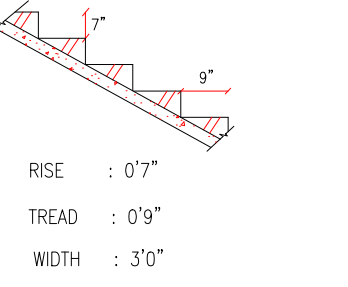
STAIRS DETAILS
