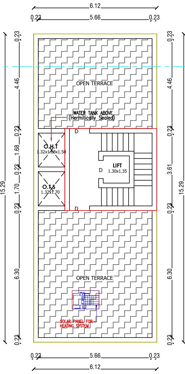
TERRACE FLOOR PLAN (PROPOSED)
