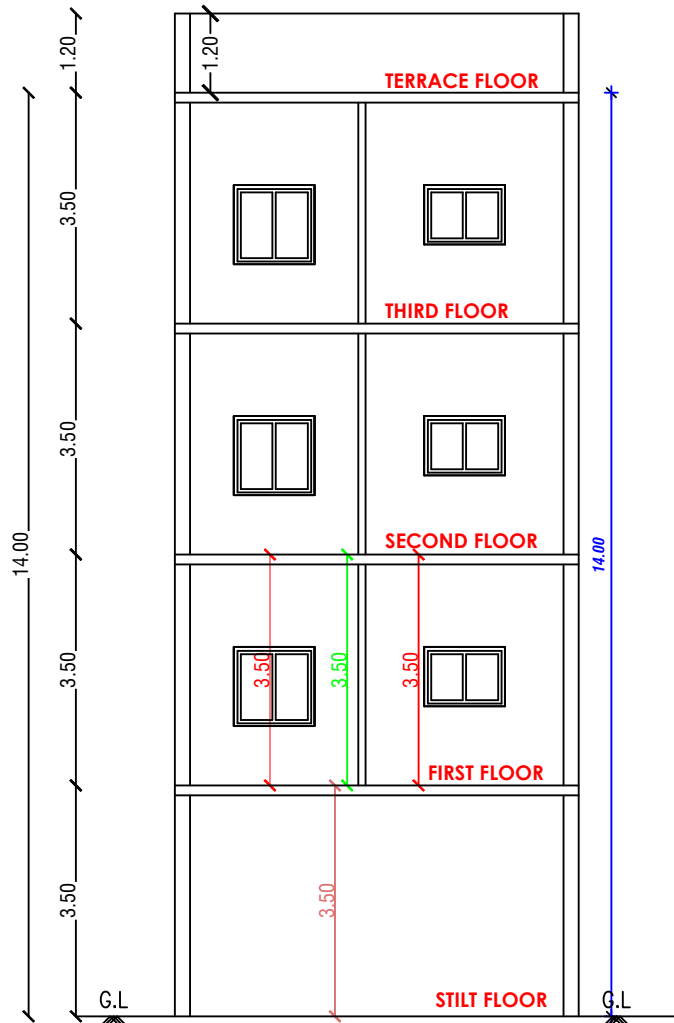
SECTION 'X-X' (PROPOSED)
