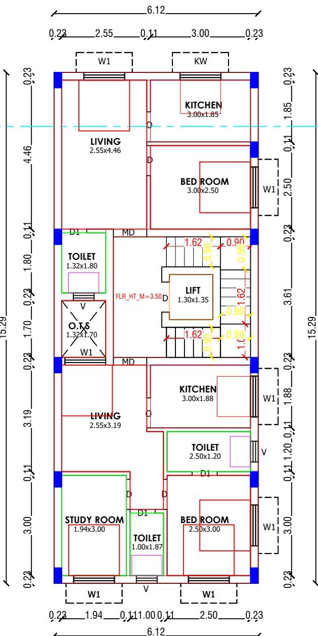
FIRST, SECOND & THIRD FLOOR PLAN (PROPOSED)
