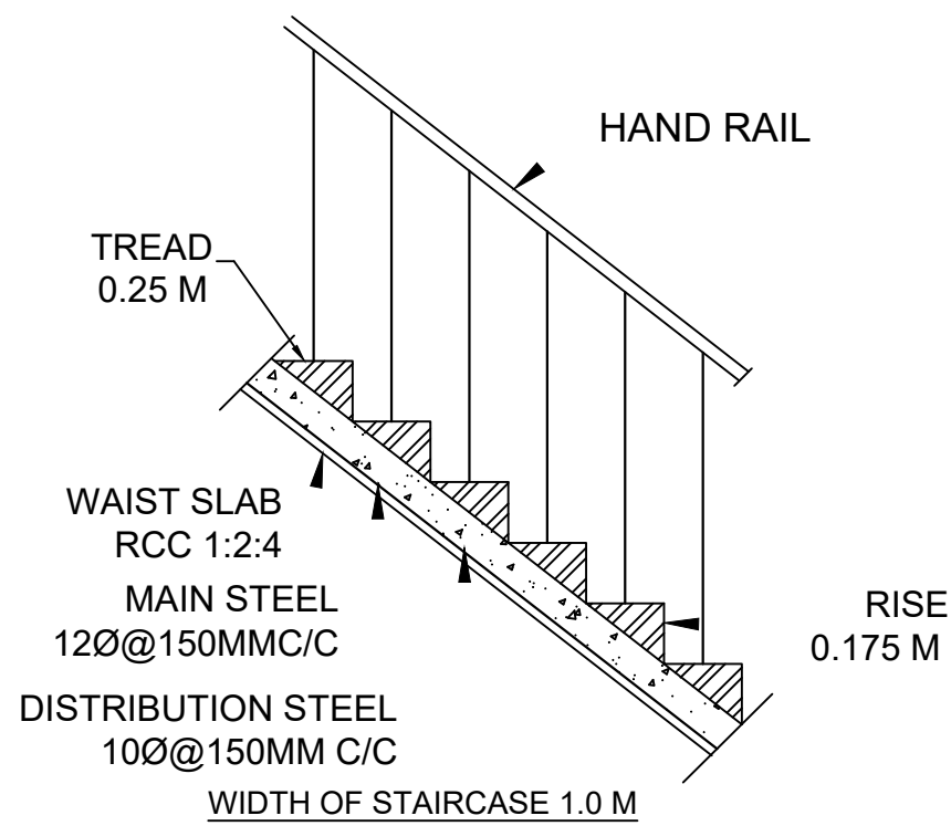
STAIR CASE DETAILS SCALE 1:300
