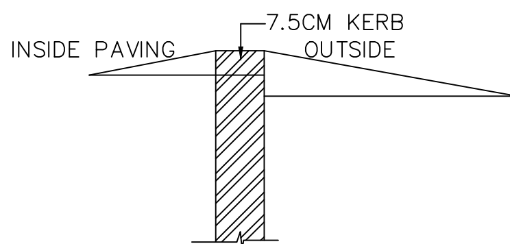
SECTION DWARF WALL SECTION
