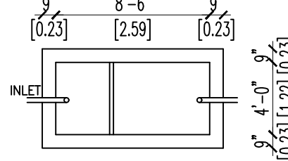
DETAILS OF SEPTIC TANK
