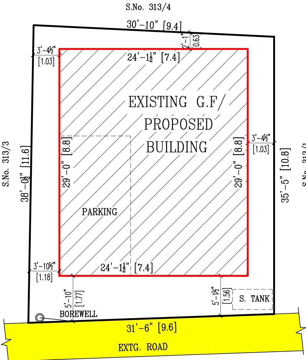
SITE PLAN
