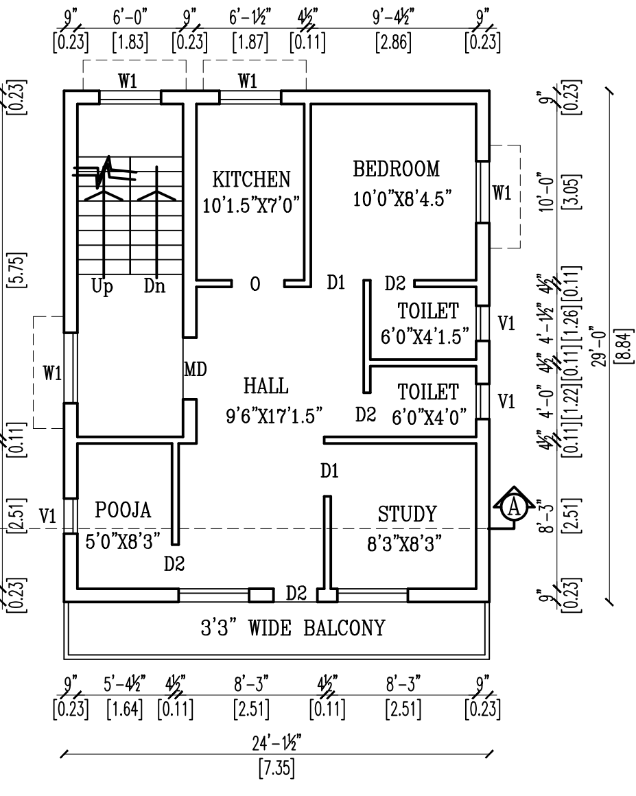
PRO. FIRST / SECOND FLOOR PLAN
