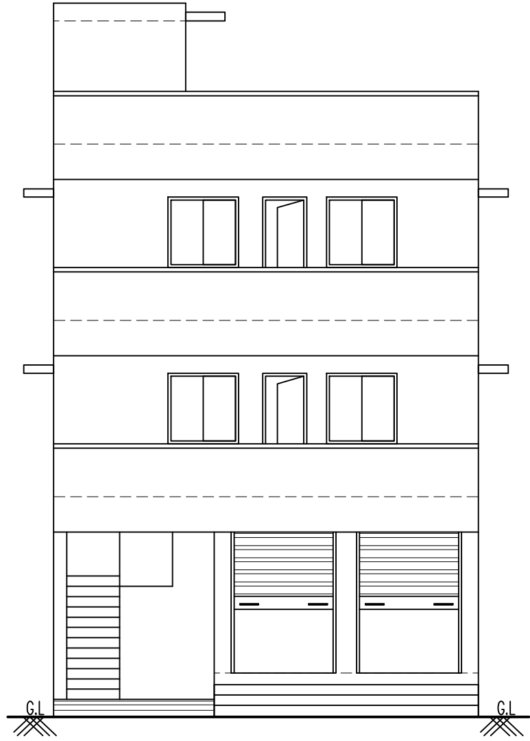
FRONT ELEVATION
