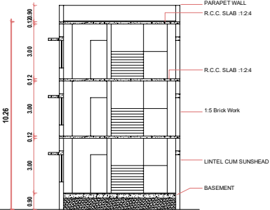
CROSS SECTION-A-B'
